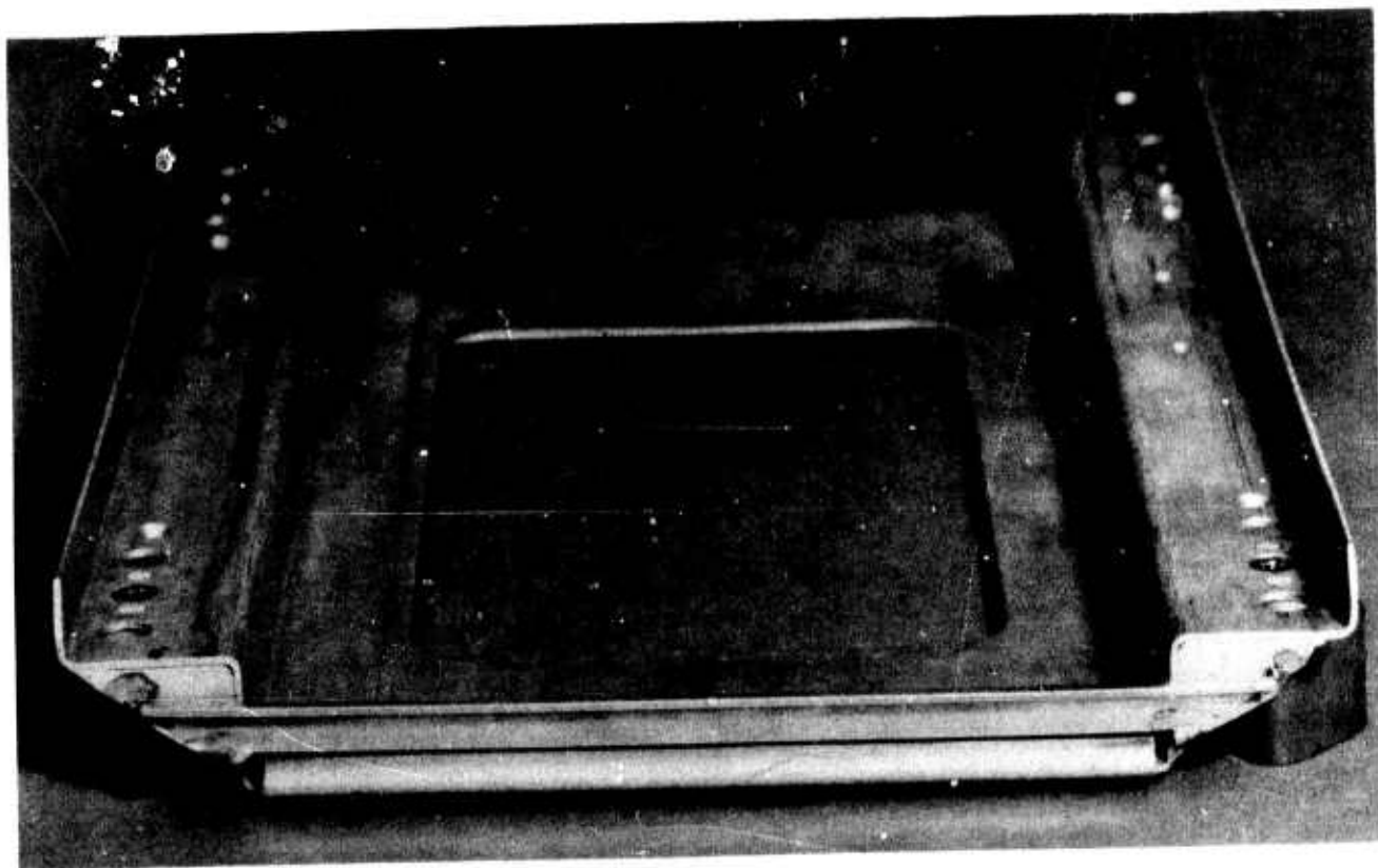
Figure 57. Mounting Tray With Stiffening Member Added
