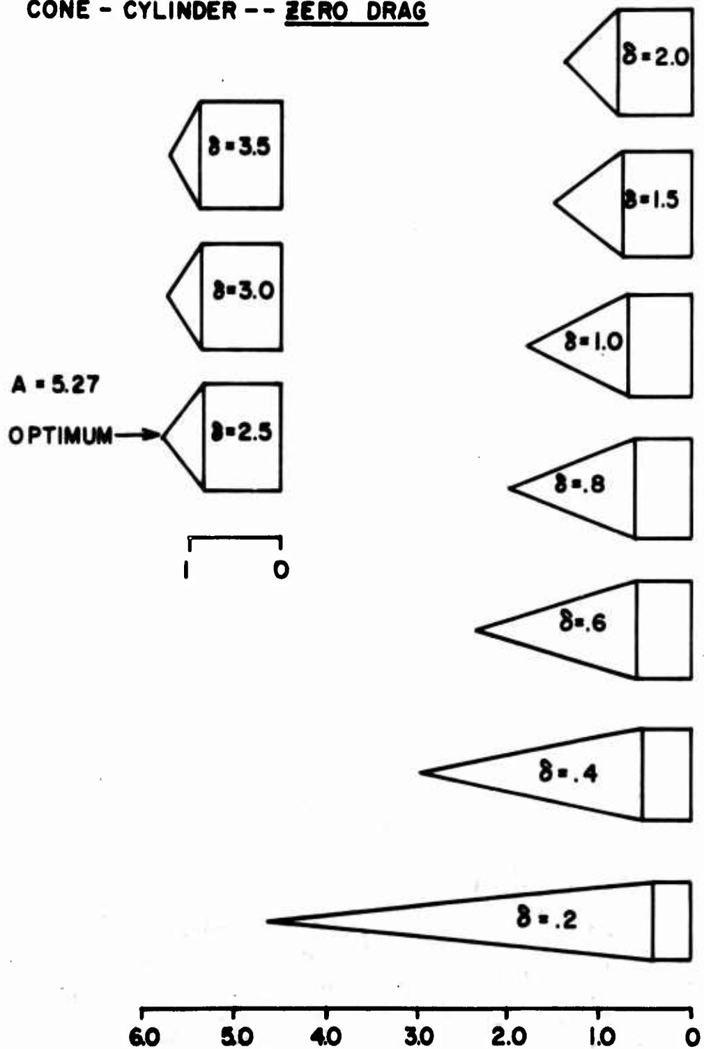
Figure 6. Series of Cone-Cylinders Fulfilling Condition a(A)/ak = 0 , with C_{D0} = 0 .
