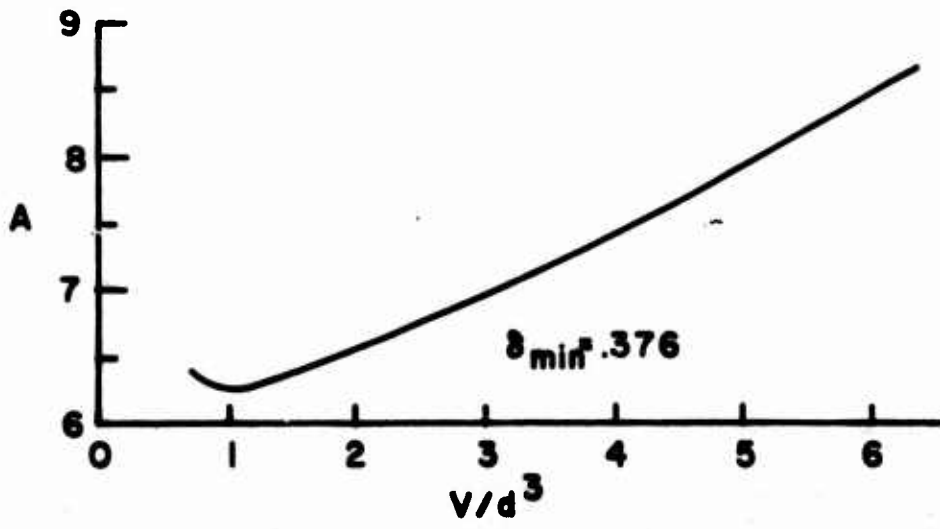
Figure 7. Variation of Cone-Cylinder Surface for Fixed Volume and Fixed Diameter.
