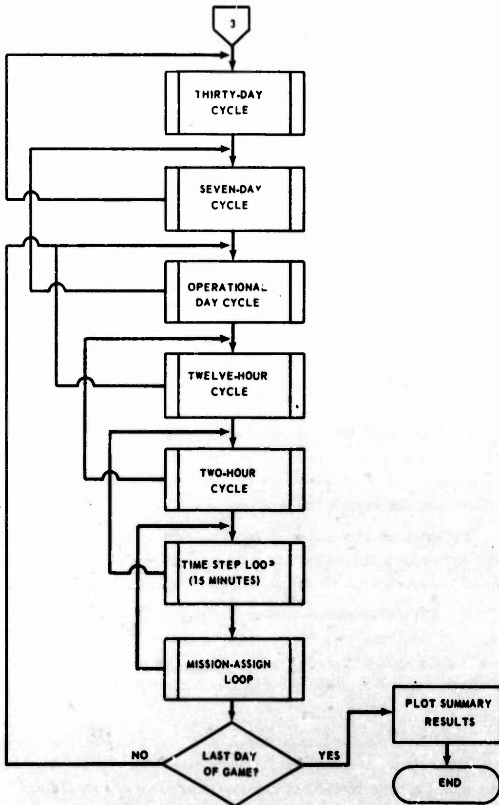
Fig. 1—EPIC Time Resolution Hierarchy
