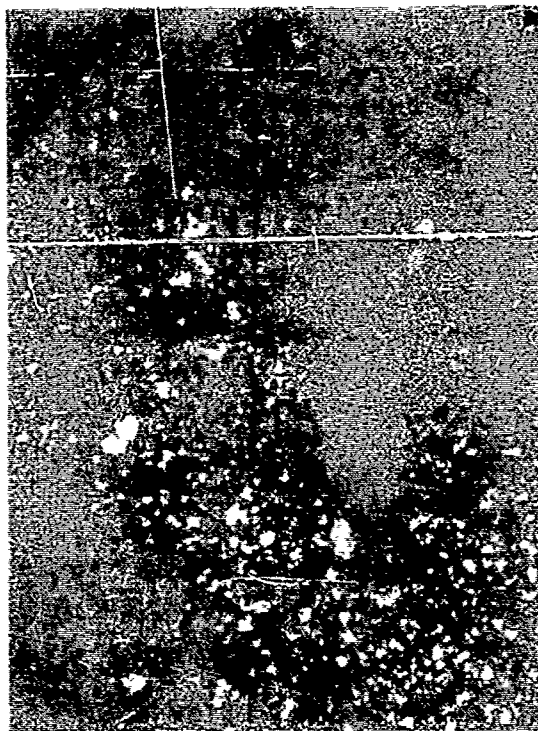
Fig. 27. \text{Ge}_7\text{Se}_7\text{As} coated KBr, after water tested. note coating is cracked.
