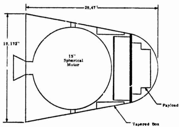
Fig. 5 NOSE CONE CONFIGURATION
