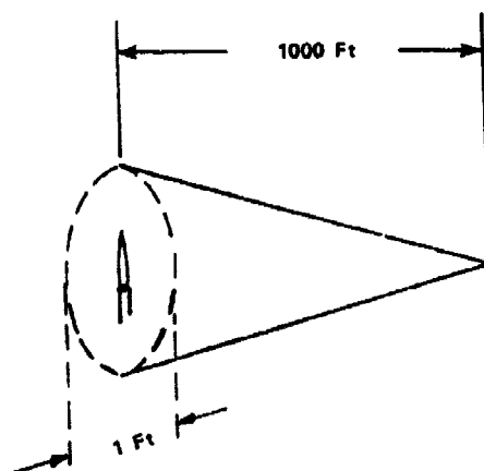
Figure 3. Definition of Field Of View
