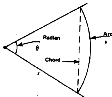
Figure 1. Definition of Radian
