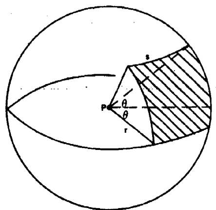
Figure 2. Definition of Steradian
