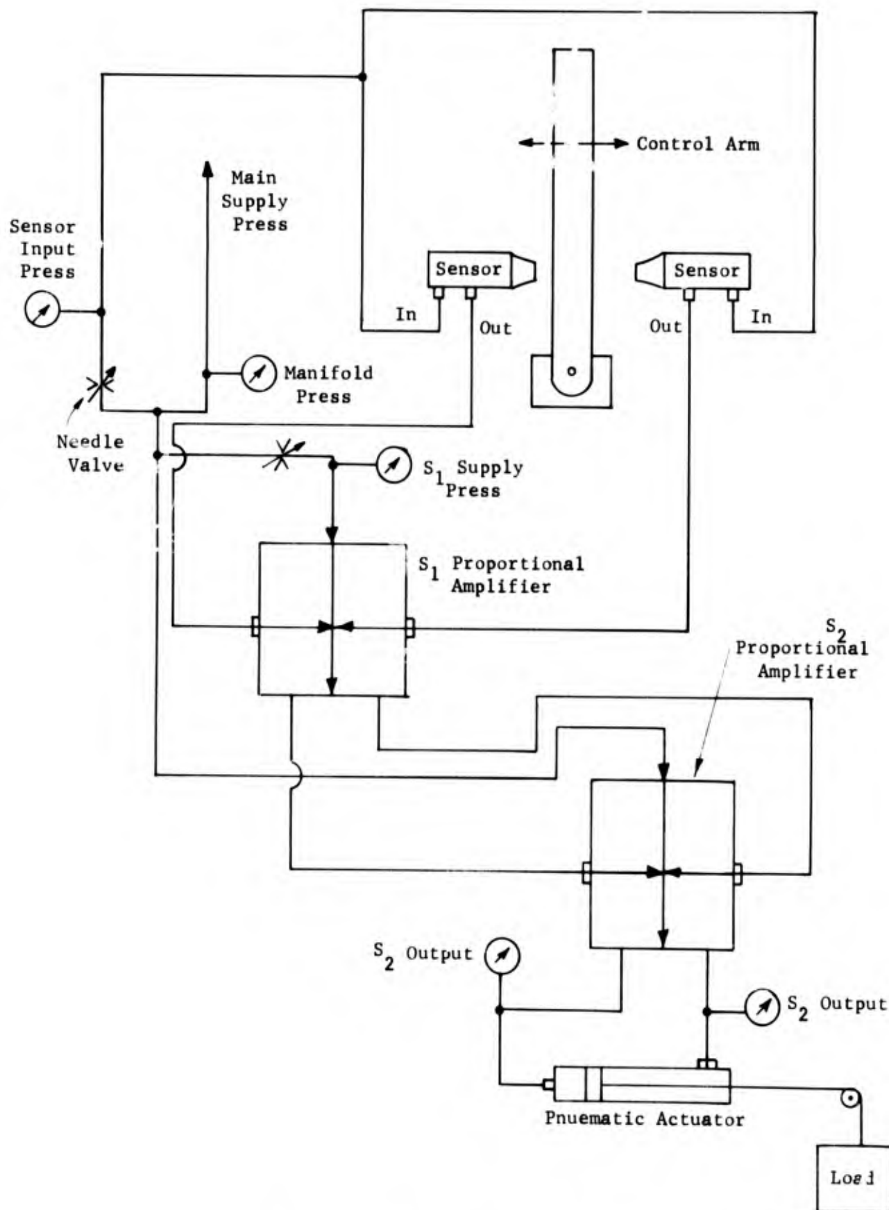
Figure 8. Pneumatic Actuator Control Circuit
