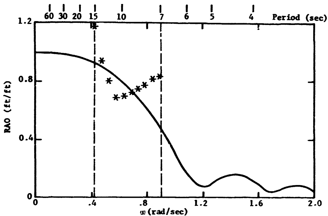
Figure E.30. Barge heave RAO for test 7.
