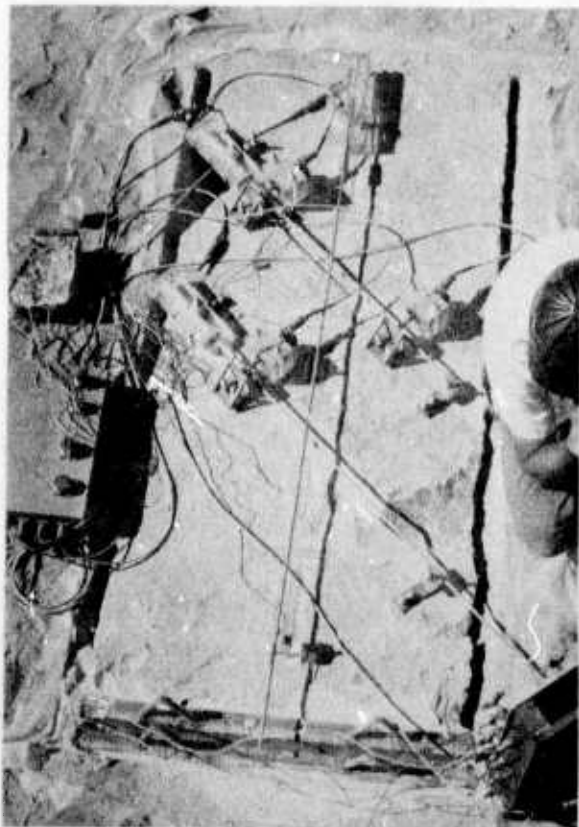
Figure 7. In-situ specimen, test 12, 3.0x6.0 feet with two joints at 45^\circ to loading axis.
