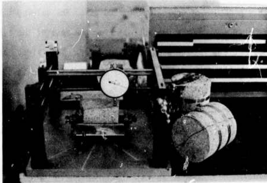
Figure 22. Joint profiler with 6-inch core ready for profiling. DCDTs are not attached.
