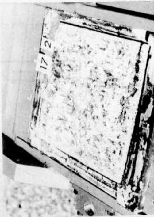
17-2 \sigma_n = 400 psi
