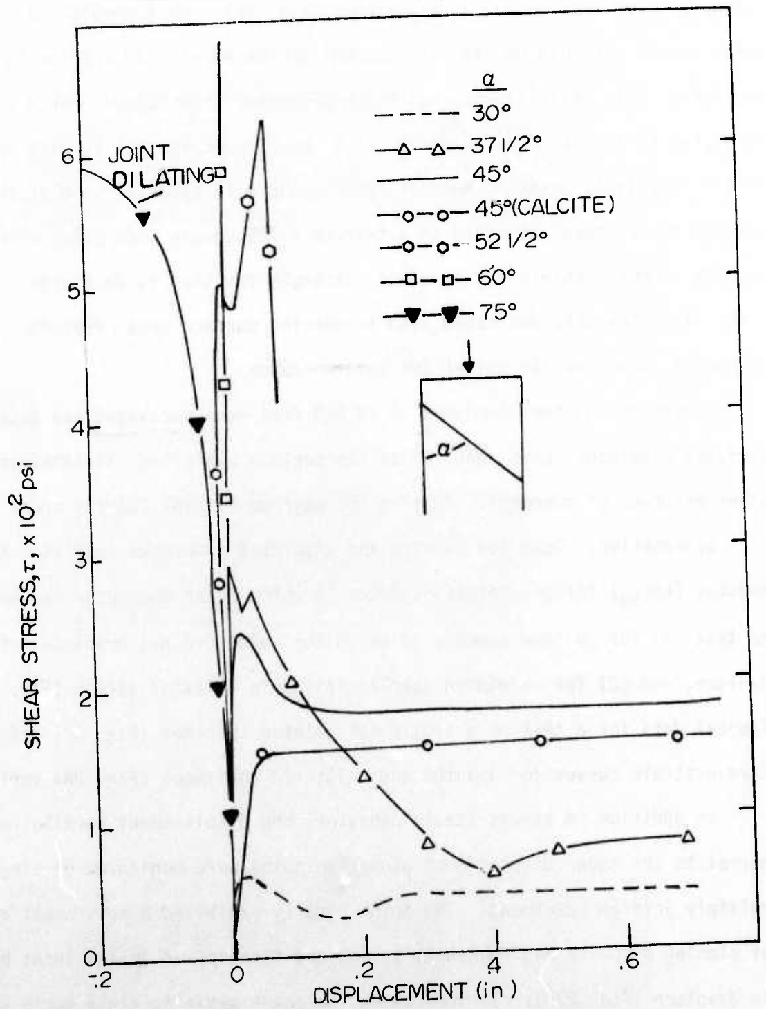
Figure 23. Shear stress versus displacement for specimens with single joint oriented at angles ranging from 30° to axis of loading.
