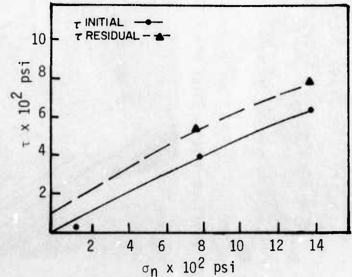
Figure 34. Frictional properties of specimen 17s at different normal stresses.
