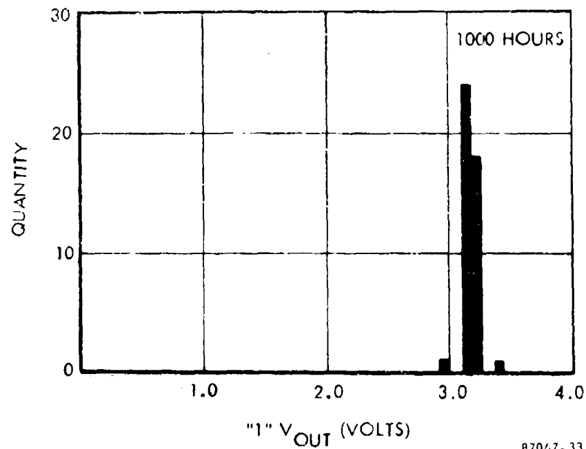
Figure 44. "1" V_{OUT} Histograms (Flip-Flop)
