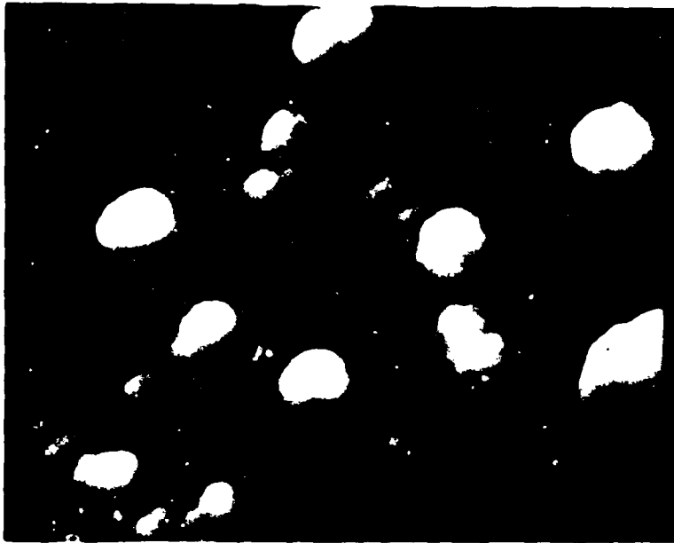
Figure 65 Device 4163 5000X Same Crack As Figure 63
