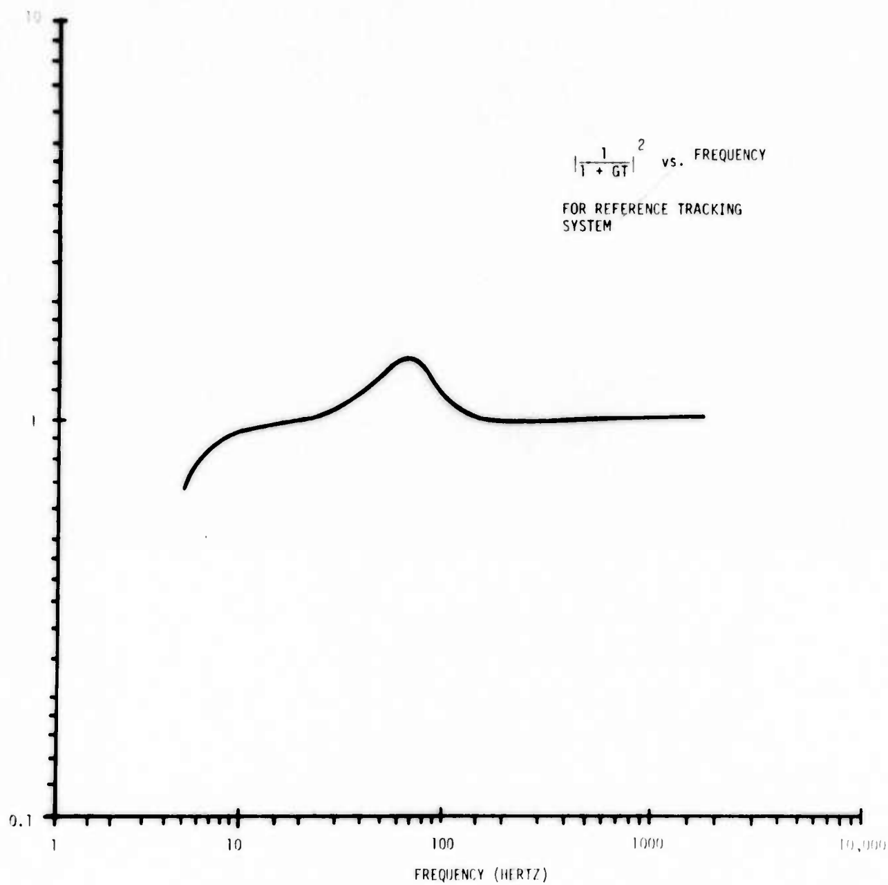
Figure 21. Rejection Function for Reference Tracking Loop
