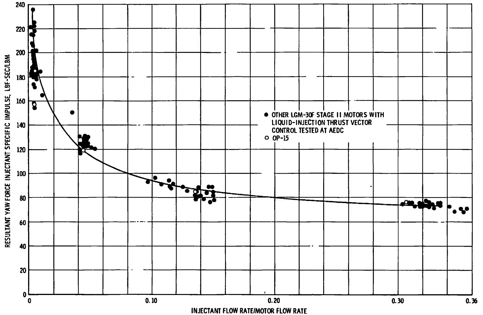
Fig. 29 Resultant Yaw Force Injectant Specific Impulse versus Injectant-to-Motor Flow Rate Ratio
