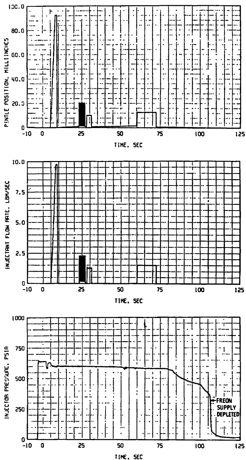
Fig. 23 Liquid-Injection Thrust Vector Control Data Summary for Injector Valve 2 (90 deg)
