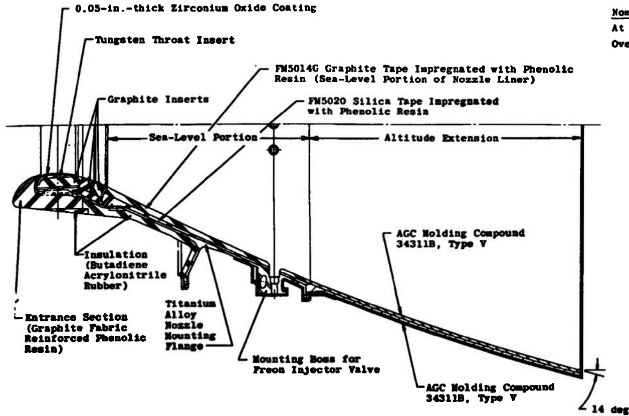
Fig. 2 Nozzle Assembly
