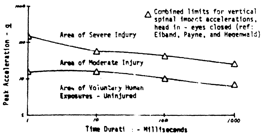
Human Tolerance Levels to Vertical Spinal - Impact Accelerations
