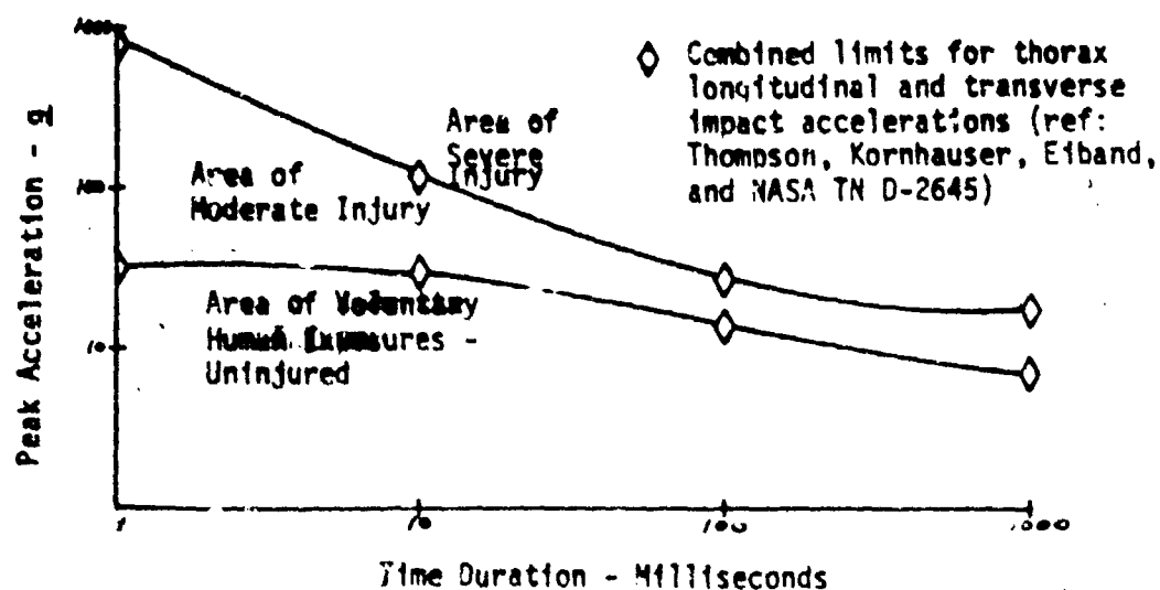
Human Tolerance Level to Thorax Transverse and Longitudinal - Impact Accel.
