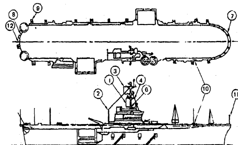
Figure 6.15. Minimum effective EM reduction plan for amphibious assault ships based on tests aboard IWO JIMA.
