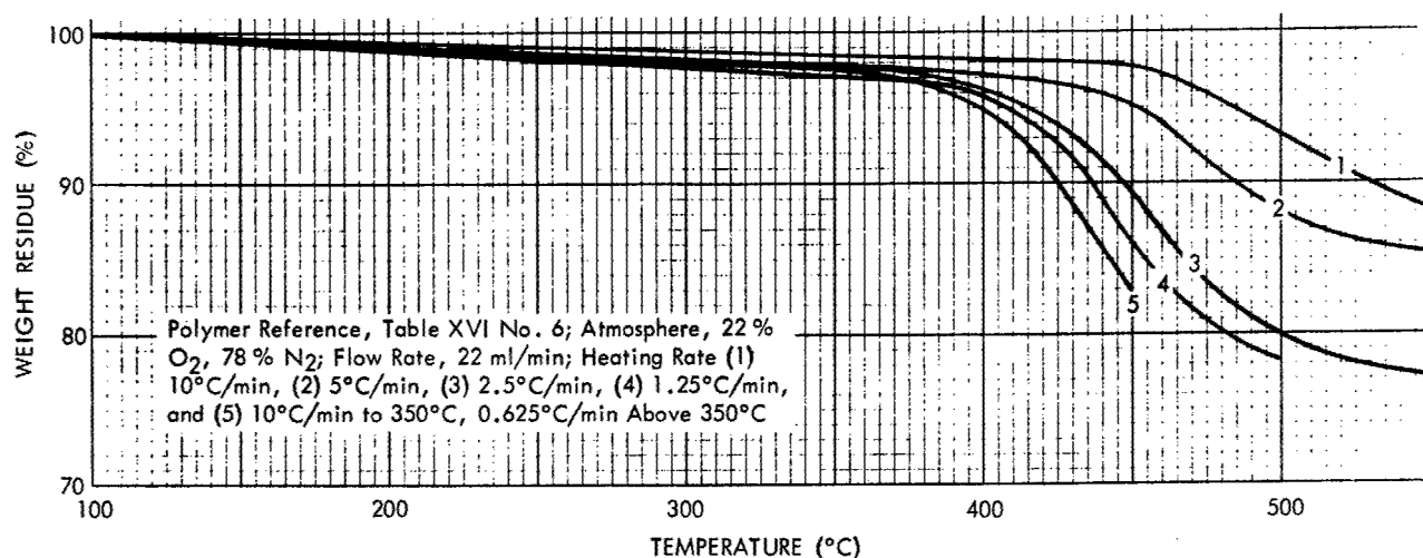
Figure 1 - Thermogravimetric Analyses at Different Heating Rates in Air of a Polymer from Oxydi- p -phenylenebis(dimethylsilanol) and Decamethyl-1,5-dioxa-3,7-diaza-2,4,6,8-tetrasilacyclooctane with 2 Mole % of p -Phenylenebis(methylvinylsilanol)
