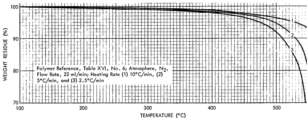
Figure 2 - Thermogravimetric Analyses at Different Heating Rates in Nitrogen of a Polymer from Oxydi- p -phenylenebis(dimethylsilanol) and Decamethyl-1,5-dioxa-3,7-diaza-2,4,6,8-tetrasilacyclooctane with 2 Mole % of p -Phenylenebis(methylvinylsilanol)
