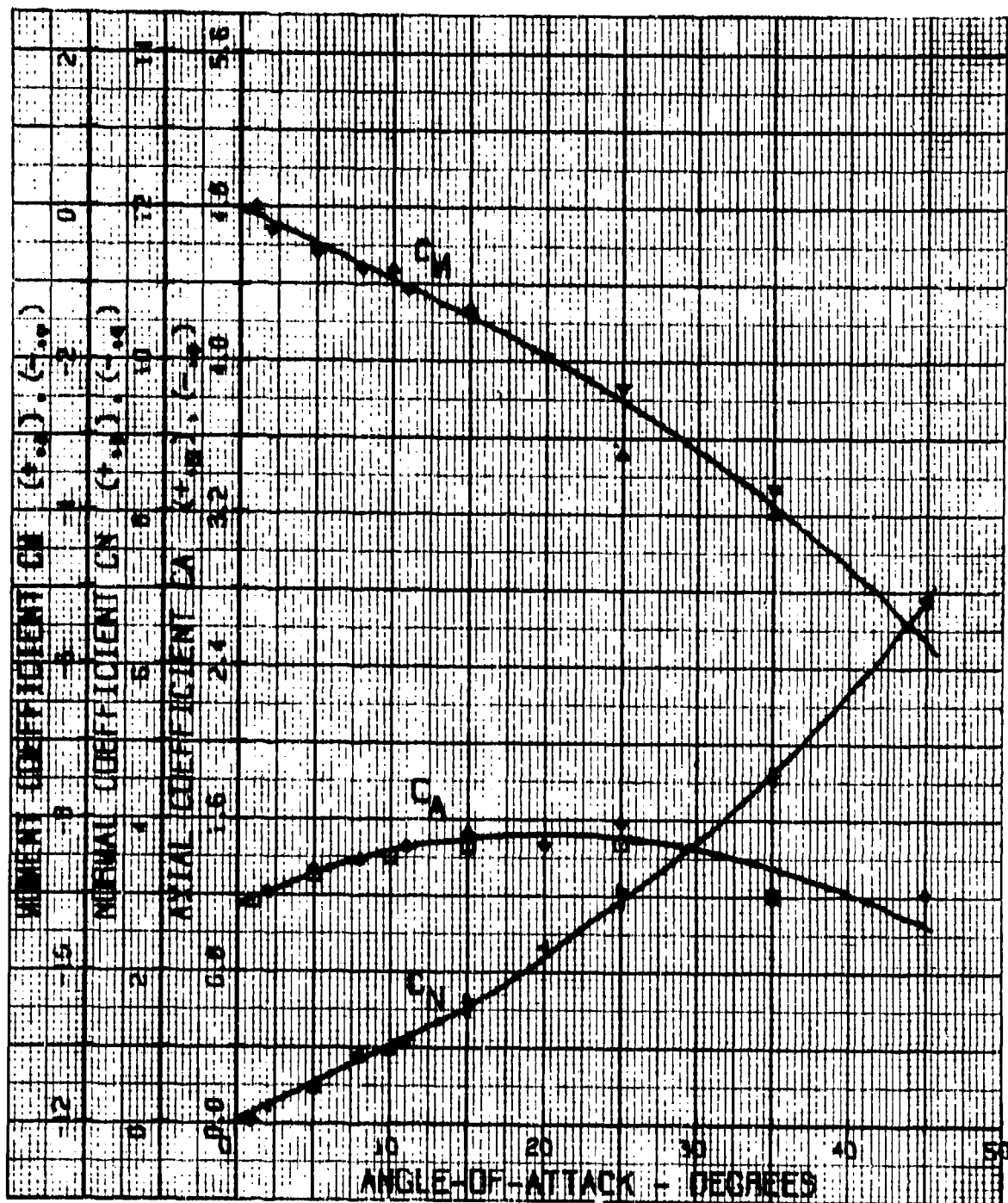
Figure 145. Graphic Static Aerodynamic Test Data: Configuration 70 (Test No. 36)
