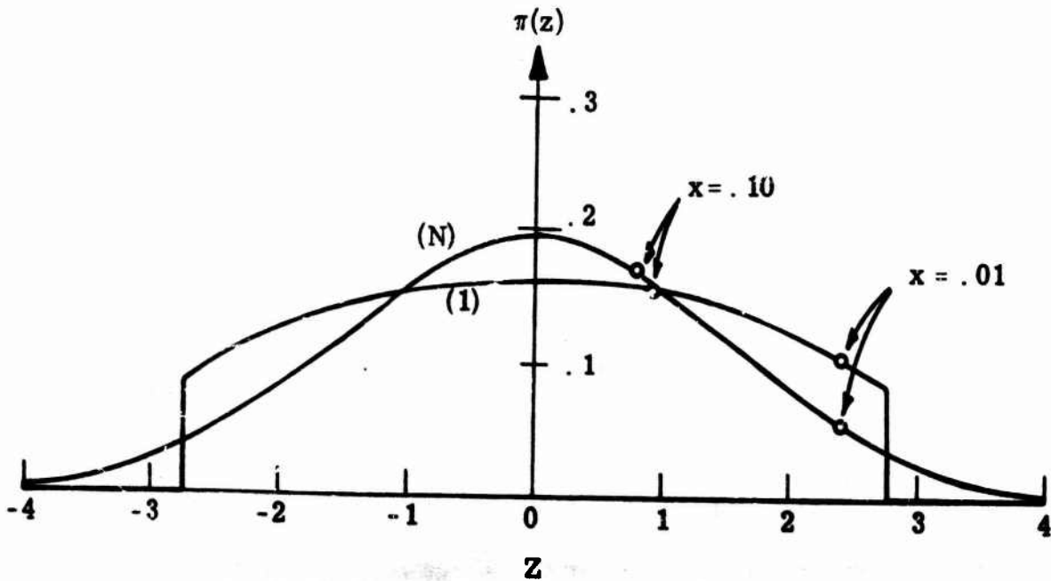
Fig. 5.15 Comparison of curves and characters for a conic and a normal ROC
