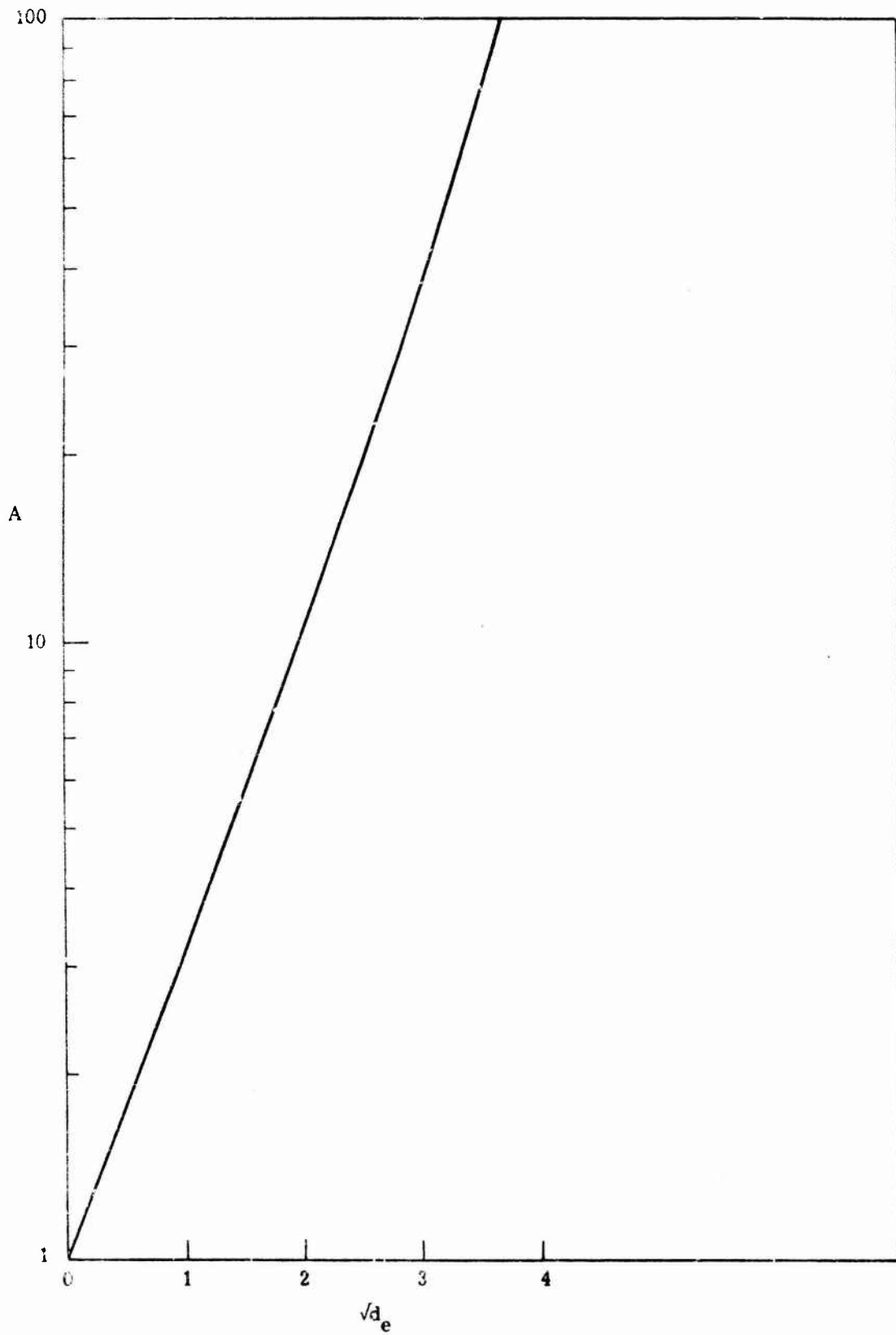
Fig. 5.5. Pure power A vs. negative diagonal normal \sqrt{d_e}
