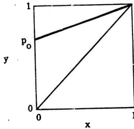
Fig. 3.6. Traditional threshold ROC
