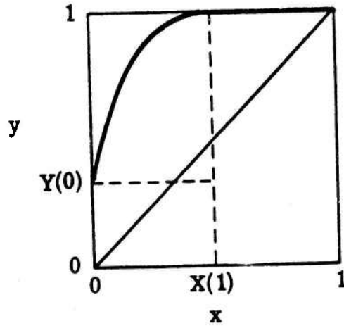
Fig. 3.5. A complete, convex, nonsingular ROC
