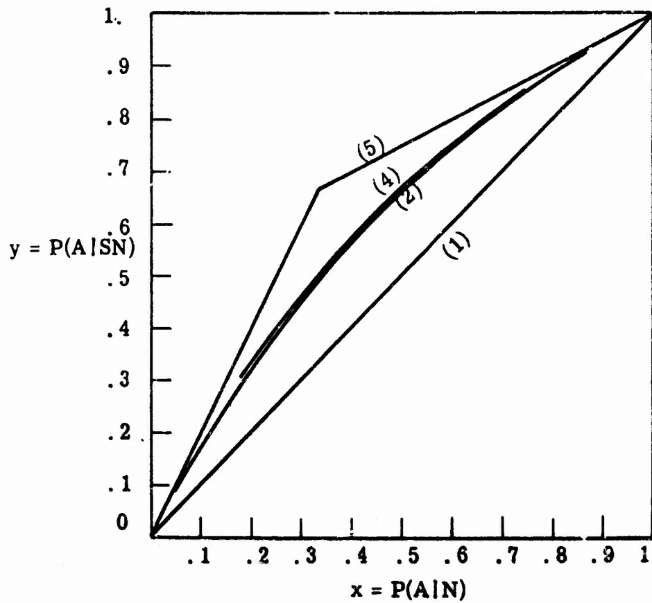
Fig. 5. 6. Symmetric conics .5 < l < 2 , |z| < .693
