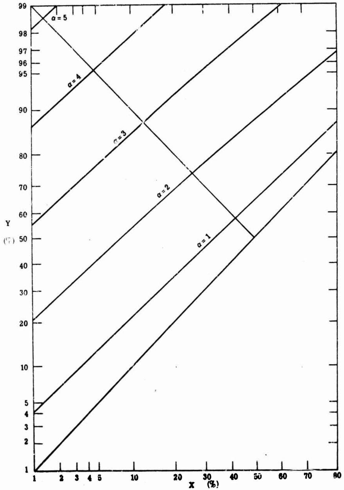
Fig. 4.5. ROC based on Q tables
