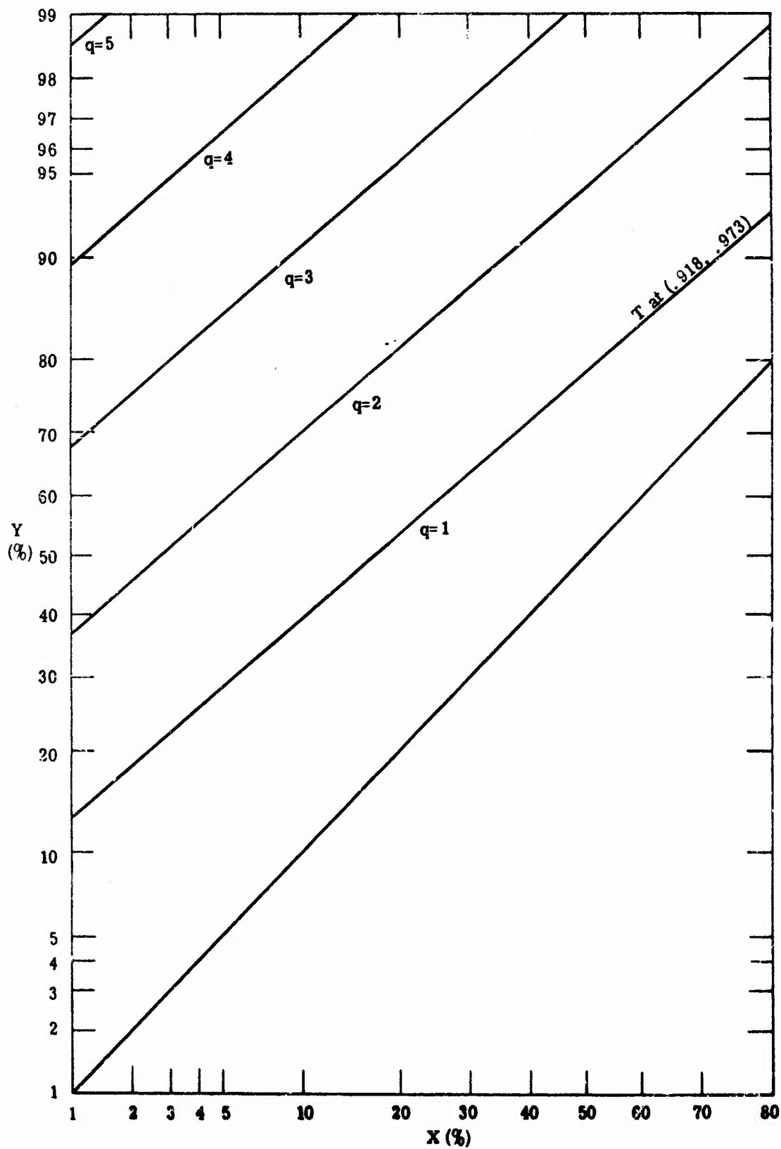
Fig. 7.8. Binormal ROC with slope s = .8 q = 1
