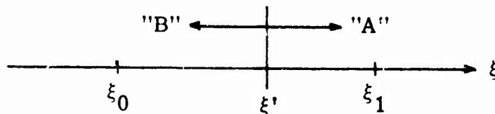
Fig. 2. 4. Arbitrary decision axis, \xi
