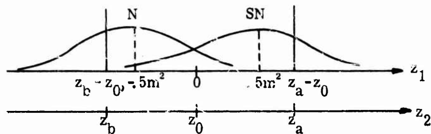
Fig. 6.1. Sketch of two z axes
