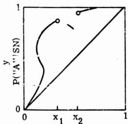
(c) Original arcs
