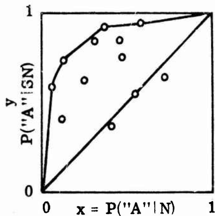
(b) Convex completion of (a)
