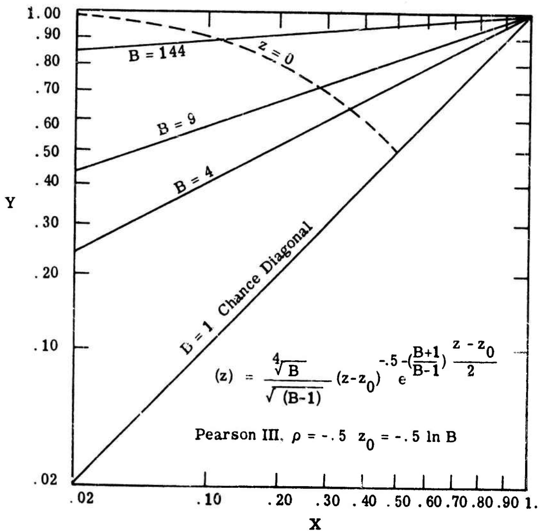
Fig. 9.2. Pearson III, \rho = -.5 , ROC curves on erf-erf paper
