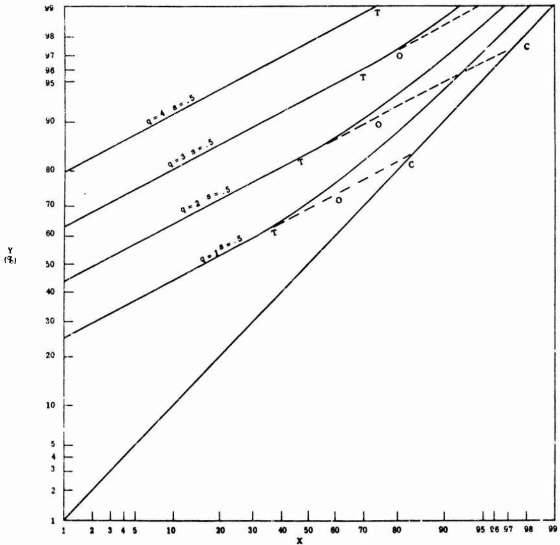
Fig. 7.9. Externally rectified binormal ROC curves
