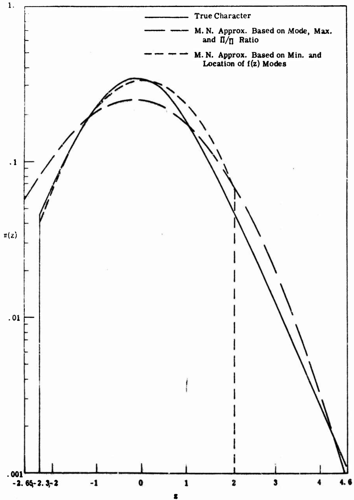
Fig. 6.5. Comparison of characters of third and fourth examples
