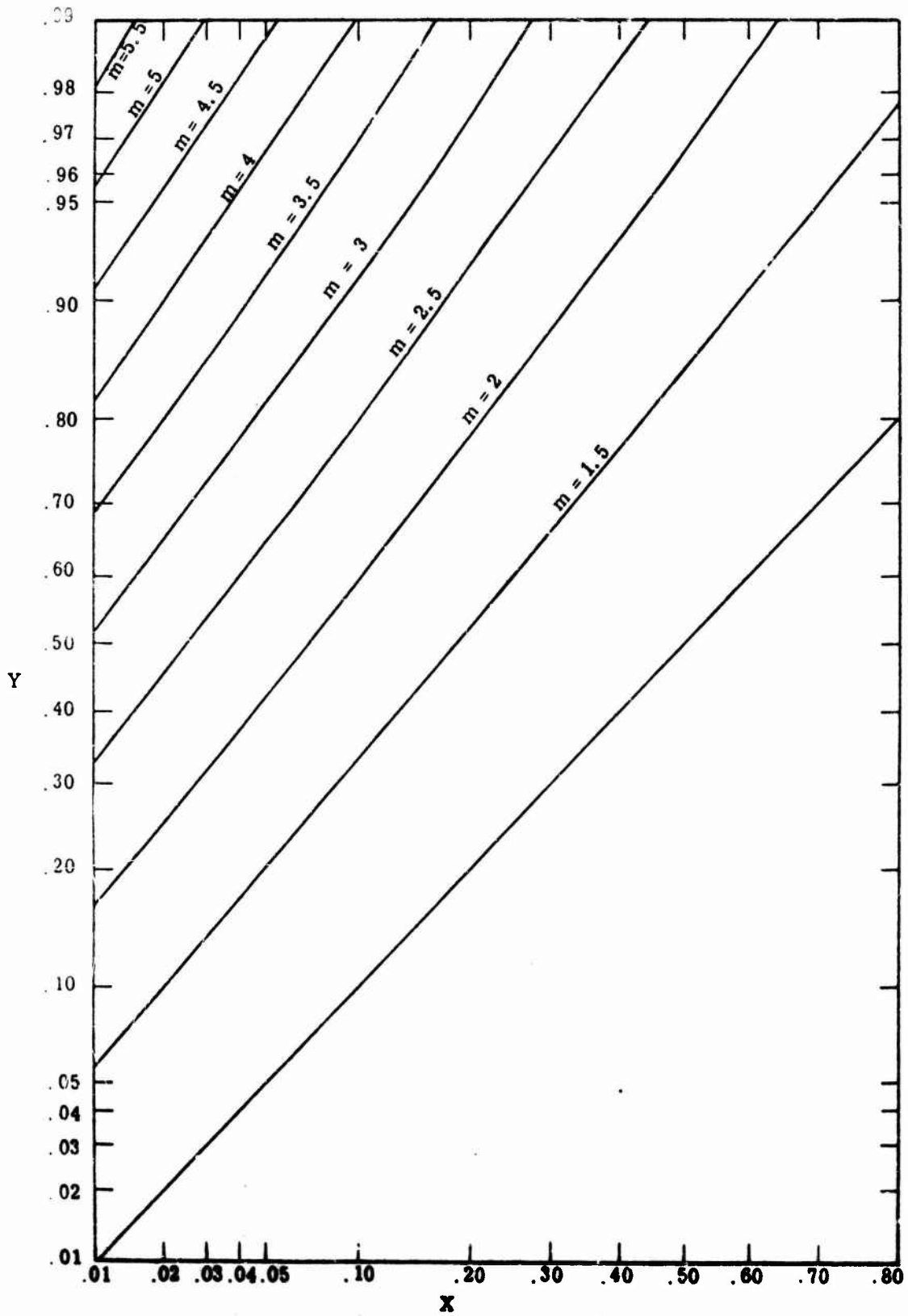
Fig. 8.5. ROC curves of Eq. 8.73
