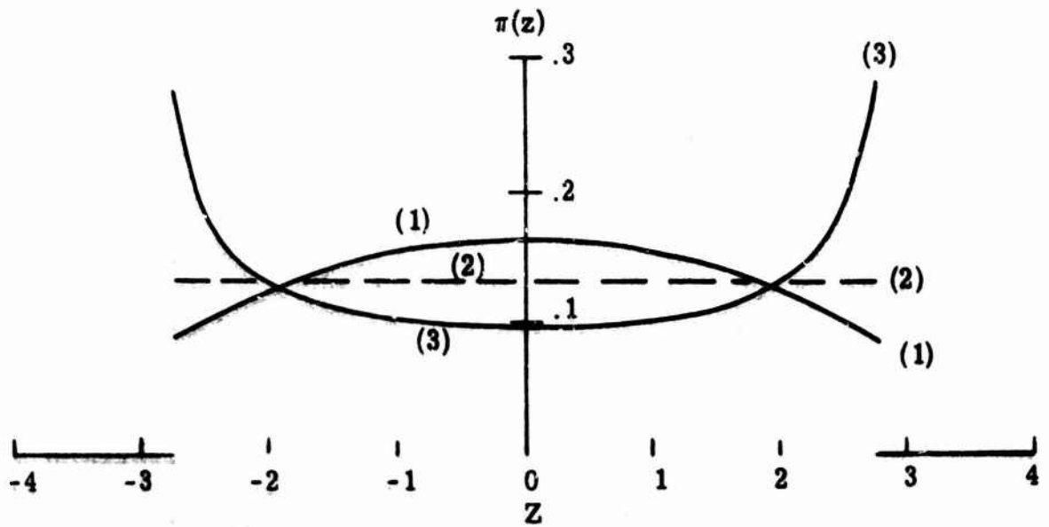
Fig. 5. 13. ROC and character for three hyperbolas
