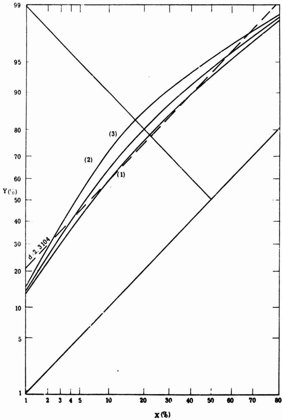
Fig. 5.14. Three hyperbolas compared to normal
