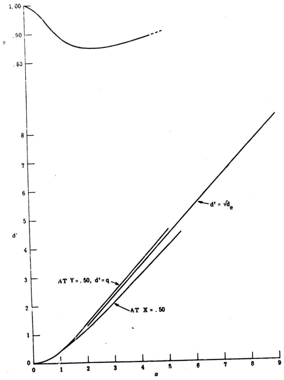
Fig. 4.6. Slope and quality values relating Q-Table ROC to normal and binormal
