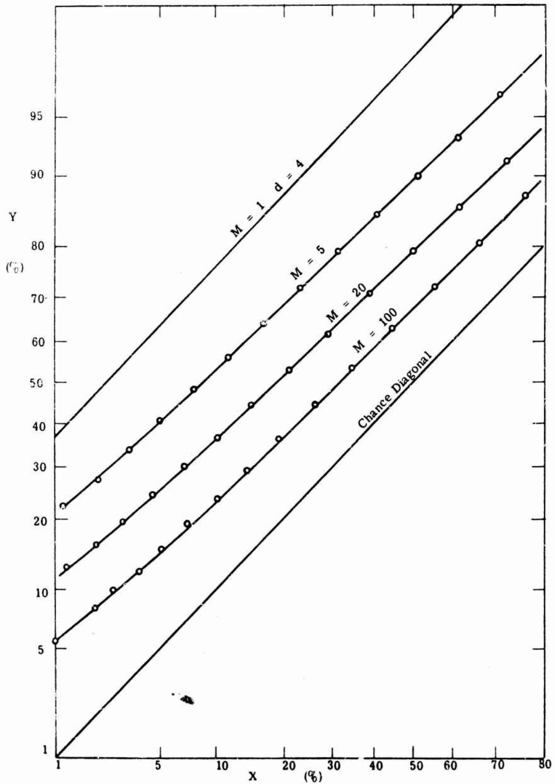
Fig. 4.9. ROC curves for M orthogonal normal signals
