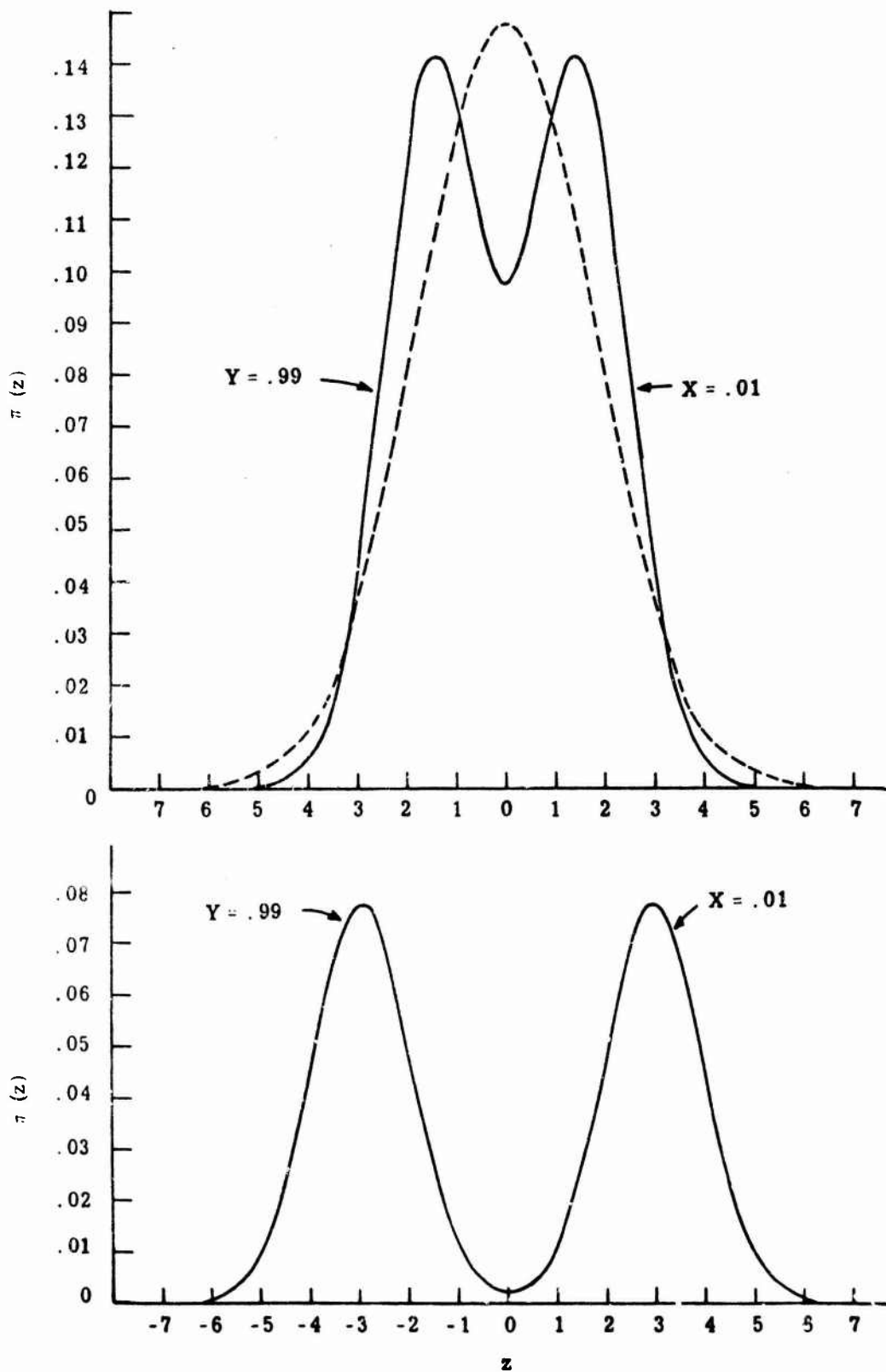
Fig. 10.3. Two multiple observer ROC characters
