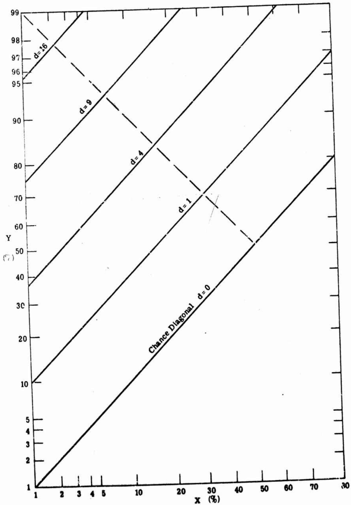
Fig. 4.2. Normal ROC on 'normal-normal' paper
