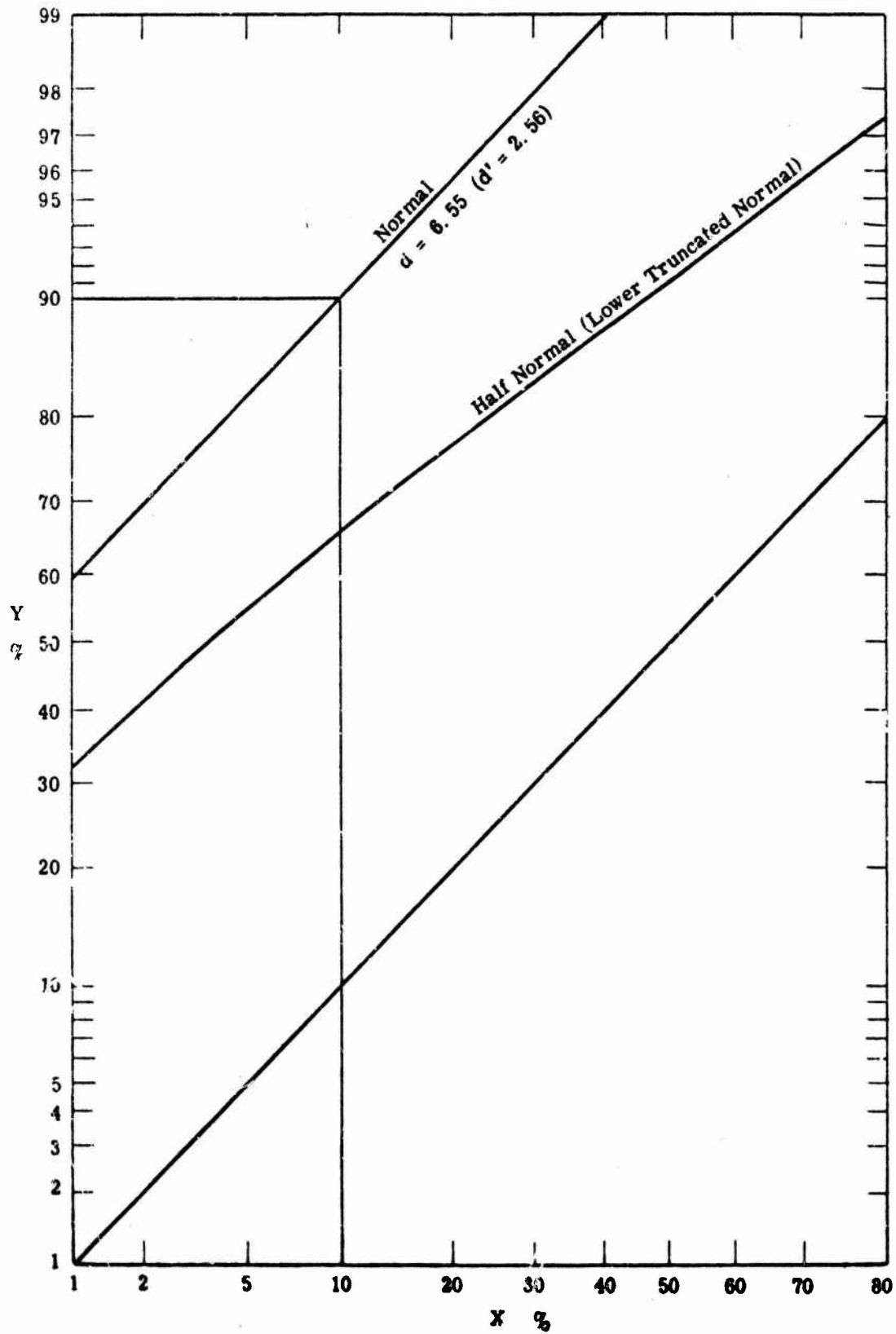
Fig. 3.4. Second example of metastatic transformation
