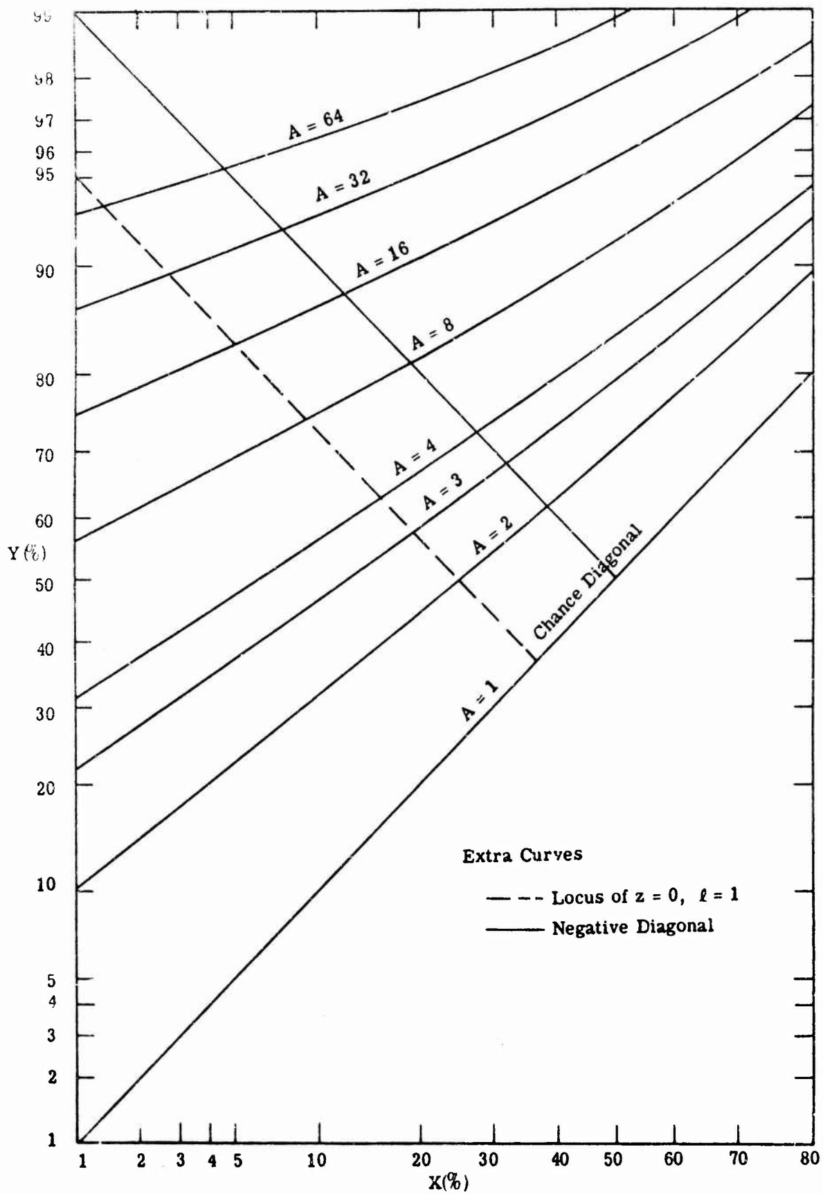
Fig. 5.3. Power ROC curves on normal-normal paper; X = Y^A
