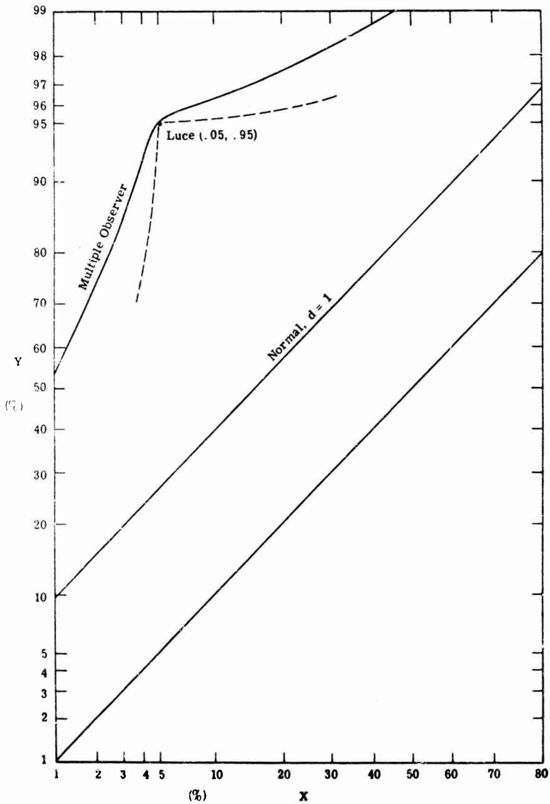
Fig. 10.4. Multiple observer ROC curve
