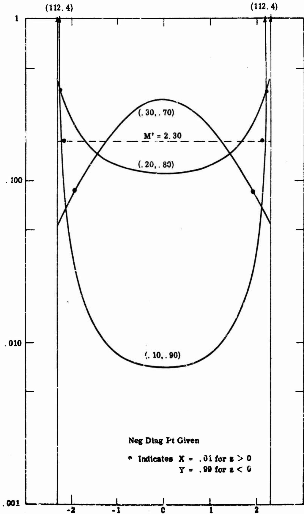
Fig. 5.21. ROC characters -2.3 \leq z \leq +2.3
