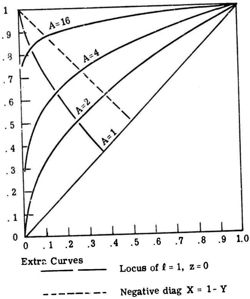
Fig. 5. 1. Power ROC curves on linear graph paper; X = Y^A
