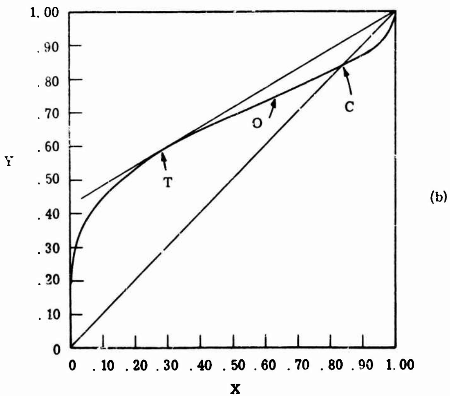
Fig. 7.5. Binormal ROC curve, q = 1 , s = .5
