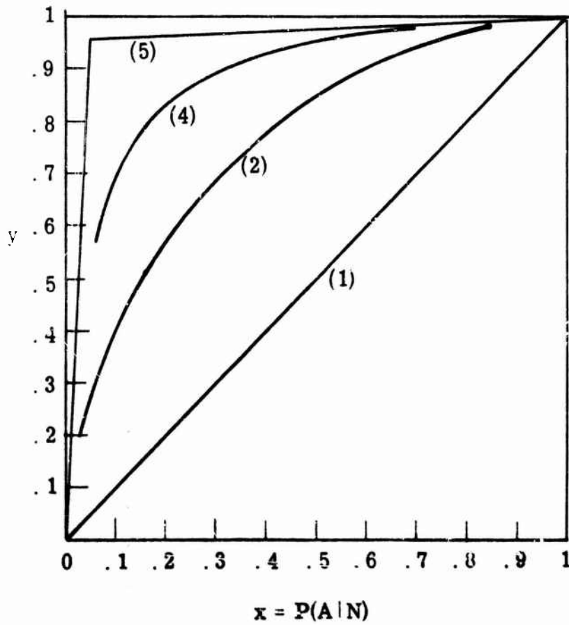
Fig. 5.9. Symmetric conics, .05 \leq \ell \leq 20 , |z| < 3.00
