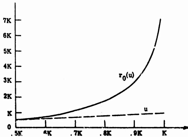
Fig. 10.9. Rating forcing functions
