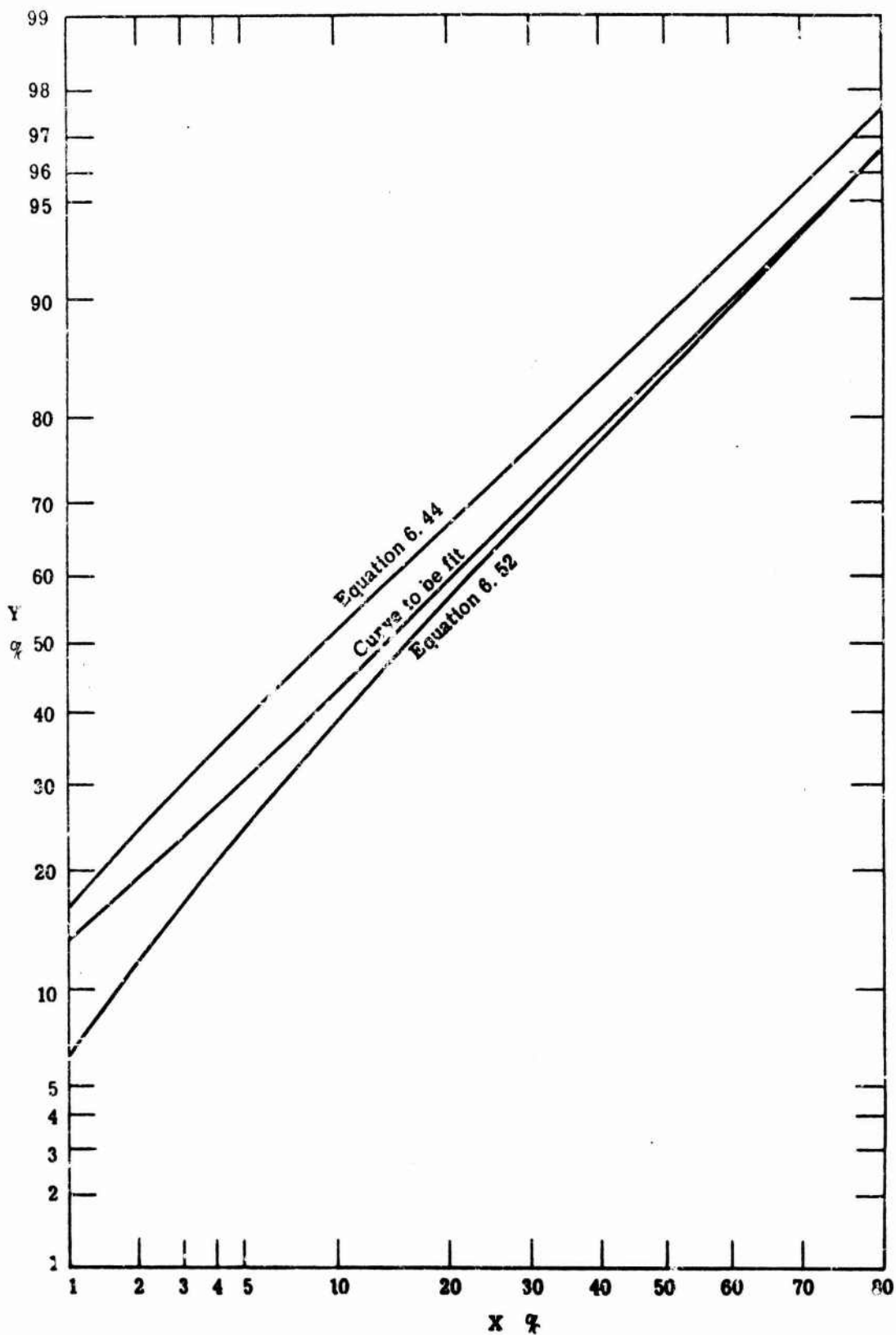
Fig. 6.4. Comparison of third and fourth examples with true curve
