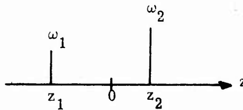
Fig. 8.3. Sketch for Luce ROC character
