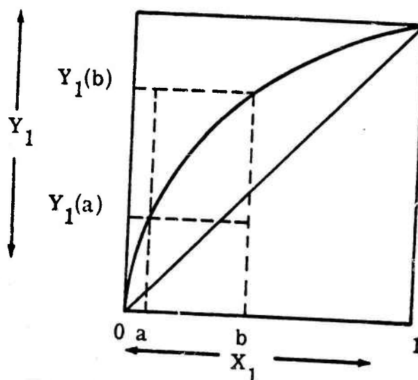
Fig. 3. 1. A particular ROC curve
