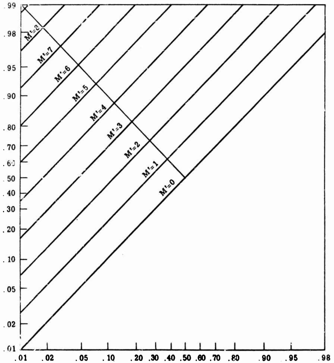
Fig. 5.18. Lor-Lor paper with lines of equal M'
