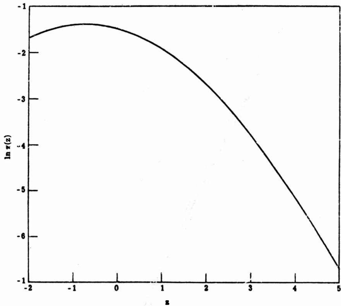
Fig. C.2. ROC character Case II, \alpha = 2
