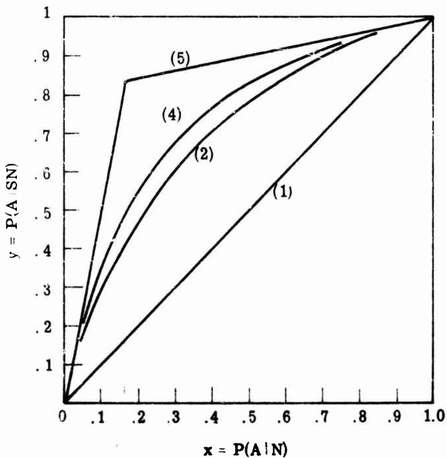
Fig. 5.7. Symmetric conics
