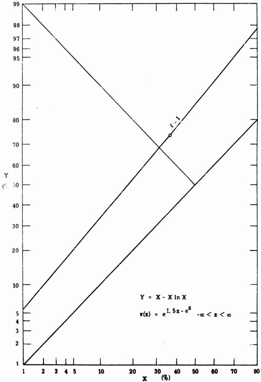
Fig. 4.8. A particular ROC curve
