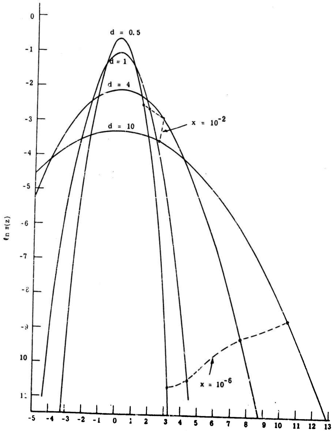
Fig. 4.4. Four normal ROC characters
