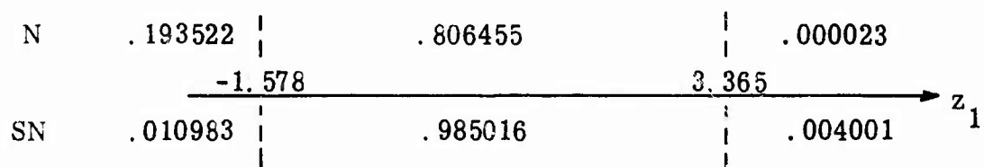
Fig. 6.3. Sketch of probabilities on original axis
