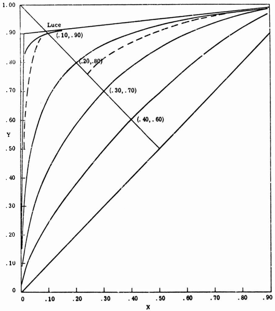
Fig. 5.23. Five asymmetric ROC curves with common terminal slope
