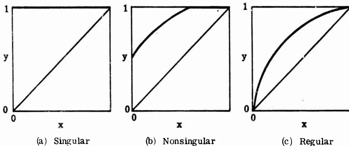
Fig. 2.3. Illustrating singularity for complete convex ROC curves
