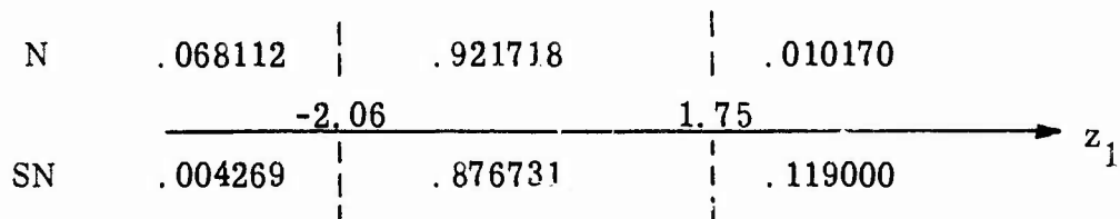
Fig. 6.6. Sketch of probabilities on original axis
