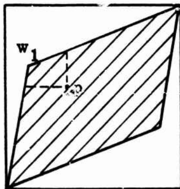
Fig. 1.5. Convex closure of a point, its opposite, and chance
