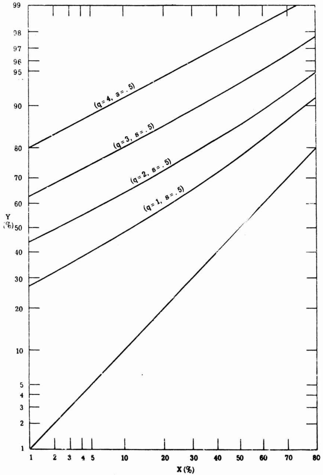
Fig. 7.12. Binormal ROC curves, internally rectified
