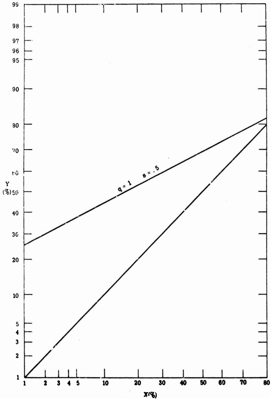
Fig. 7.4. A binormal ROC curve
