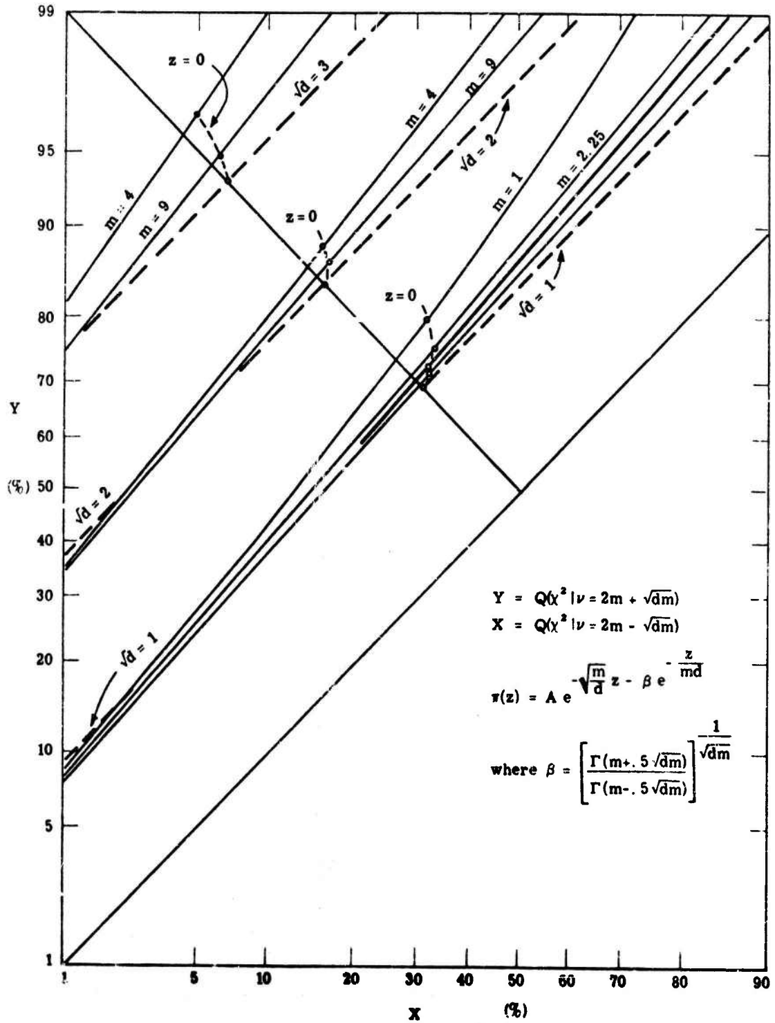
Fig. 8.4. Fisher-Tippett ROC curves
