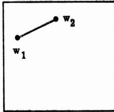
Fig. 1.3. The "convex closure" of two points
