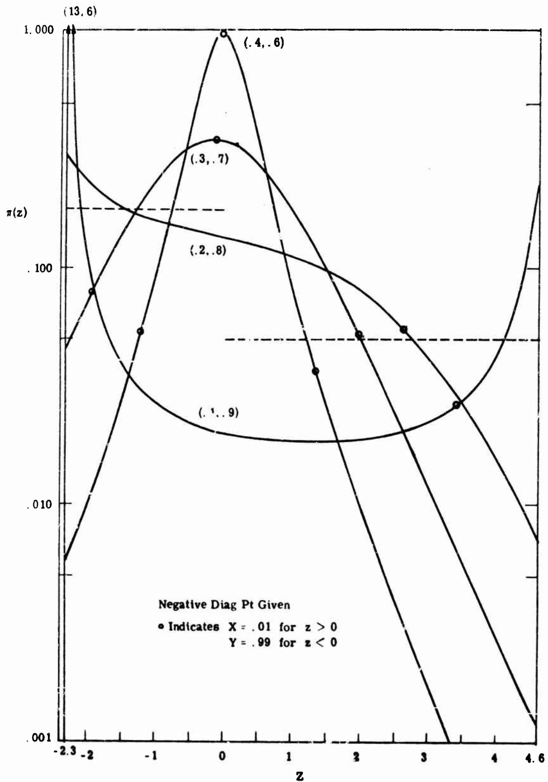
Fig. 5.24. ROC characters -2.3 \leq z \leq +4.6
