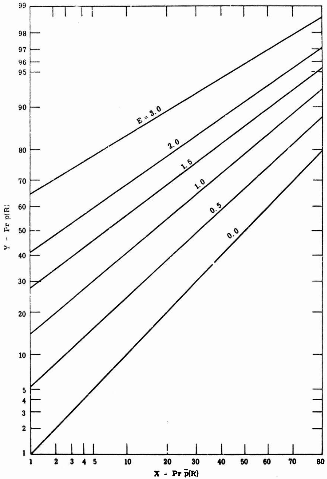
Fig. 7.1. A fan of binomial ROC curves
