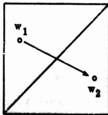
Fig. 1.4. Existence of midpoint symmetry
