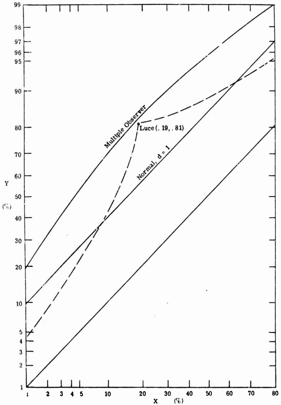
Fig. 10.2. Multiple observer ROC curve
