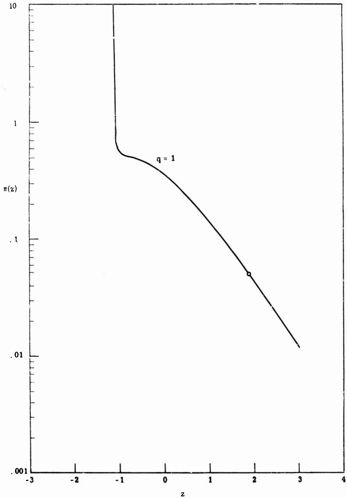
Fig. 7.10. ROC character for internally rectified binormal, q=1 , s=.8
