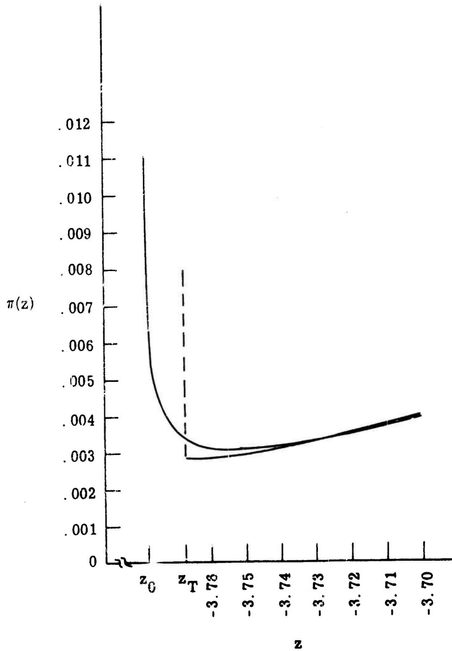
Fig. 7.11 Detail of ROC character, q=2, s=.8
