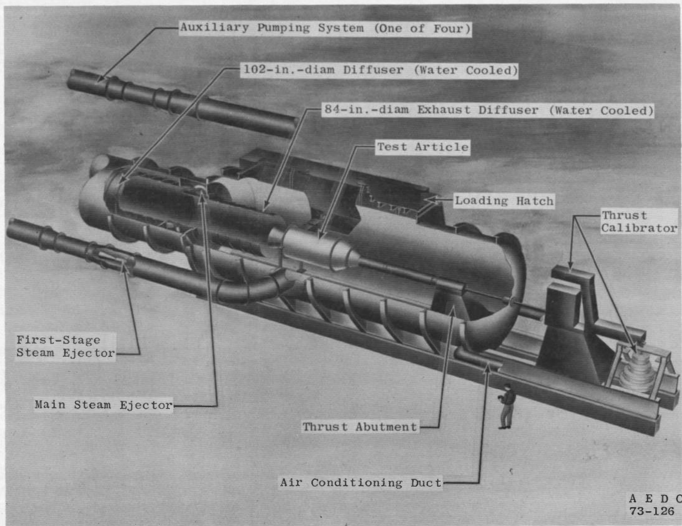
Fig. 3 Rocket Development Test Cell (J-5)
