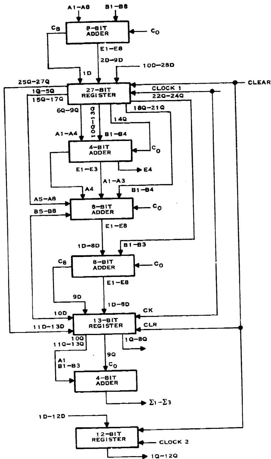
Figure 14-Adder Tree No. 1.
