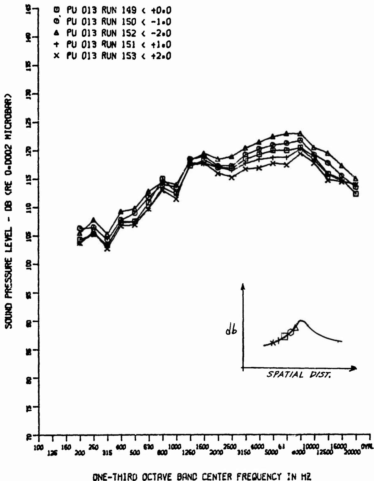
Figure 178. Comparison of Spectra in Transition Zone ( M_\infty = 10 , Re_\infty = 2.2 \times 10^6 , R_N = 0.055 )
