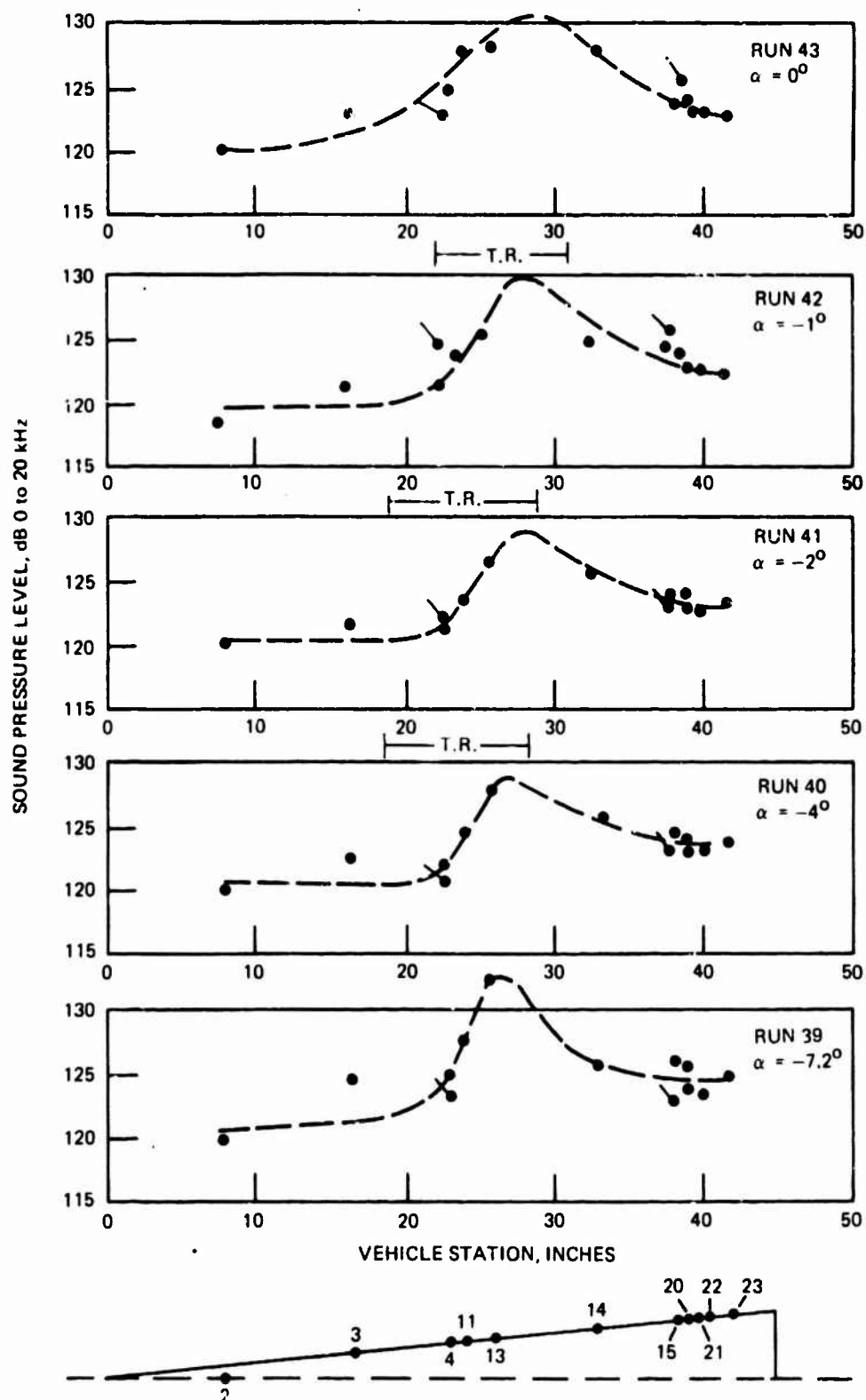
Figure 68. Fluctuating Pressure Distribution Tunnel Condition (R_{e\infty} = 3.0 \times 10^6, M_\infty = 4.0, R_N = 0.11)
