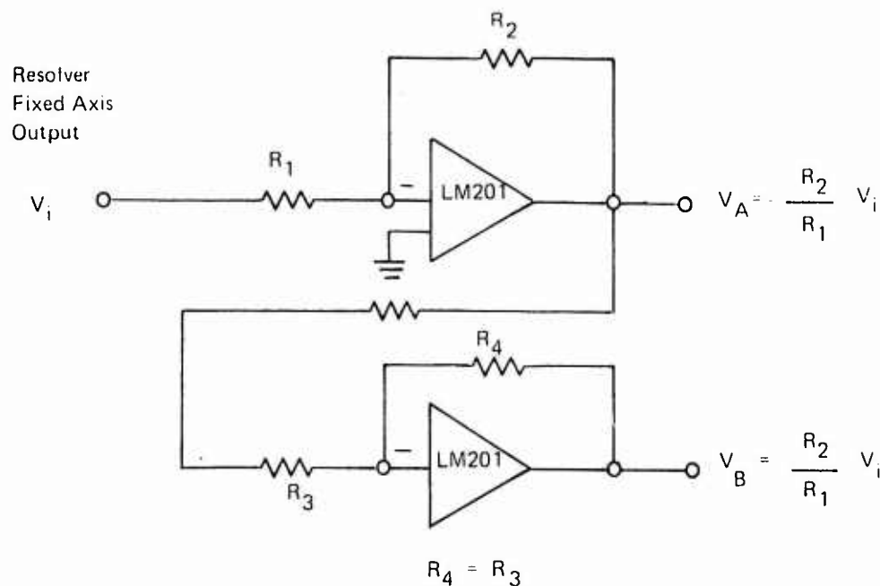
Figure 21. Fixed-Axis Amplifier
