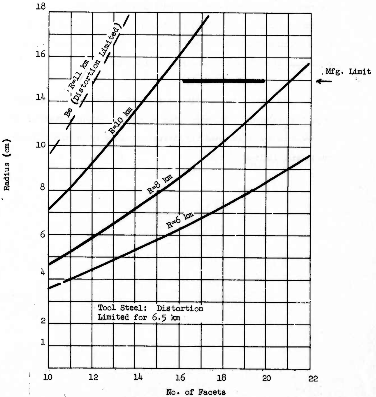
Scanner Radius Required for one-beam multifaceted system
