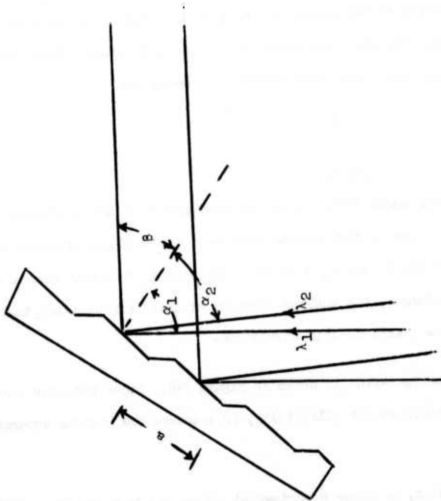
FIGURE V-3. GRATING GEOMETRY
