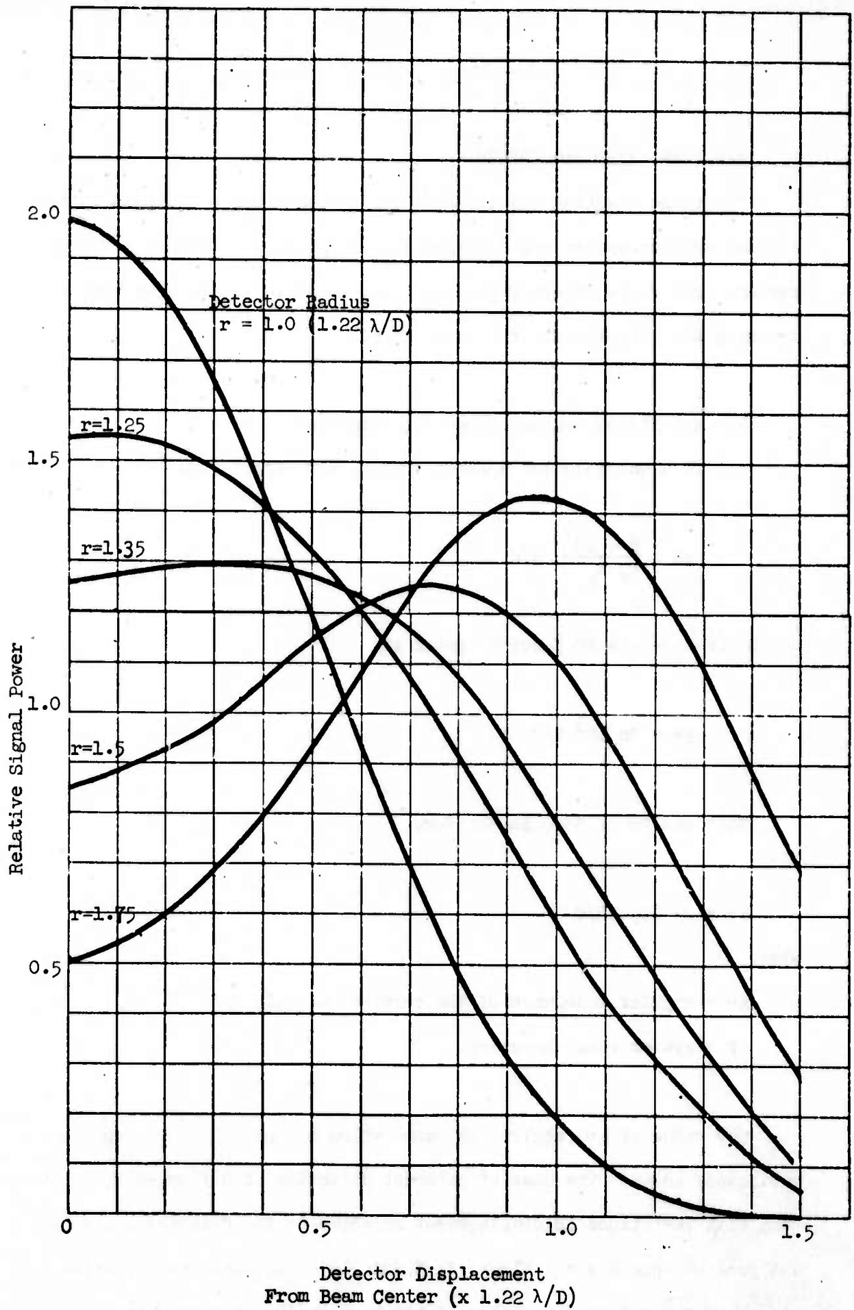
Figure II-9: Signal Power in Heterodyne Detection with Beam Center Displacement
