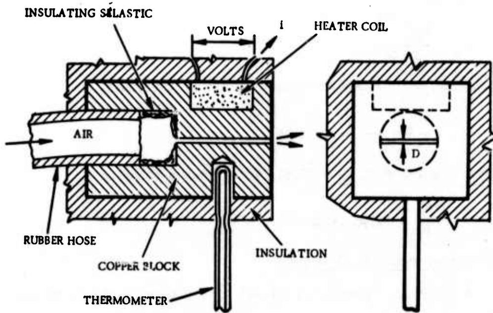
Figure II-9. Experimental Arrangement
