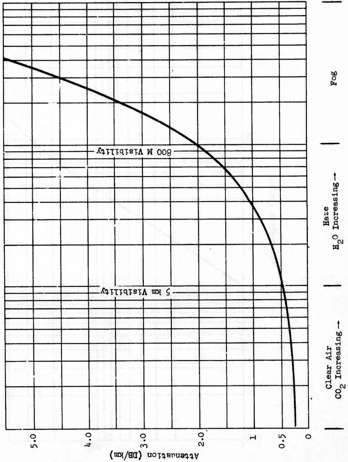
Figure II-5: Atmospheric Attenuation
