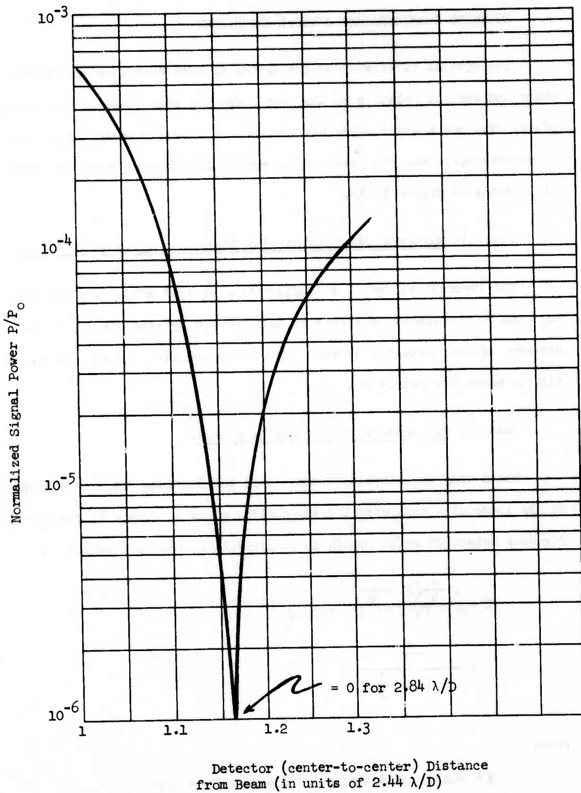
Figure II-12: Optical Cross-Talk on Adjacent Detector. Detector size = 2.44 \lambda/D ( P_0 = Signal power with detector at beam center.)
