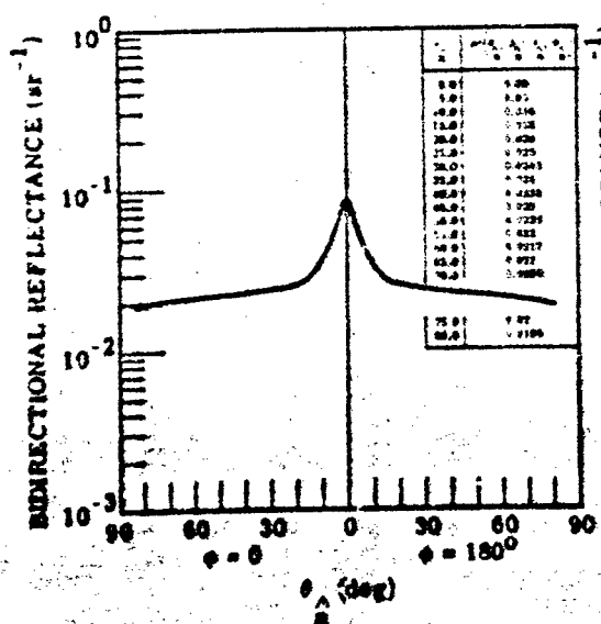
FIGURE 55. FIXED BISTATIC \rho' FOR A01456; \lambda = 1.06 \mu\text{m} .
