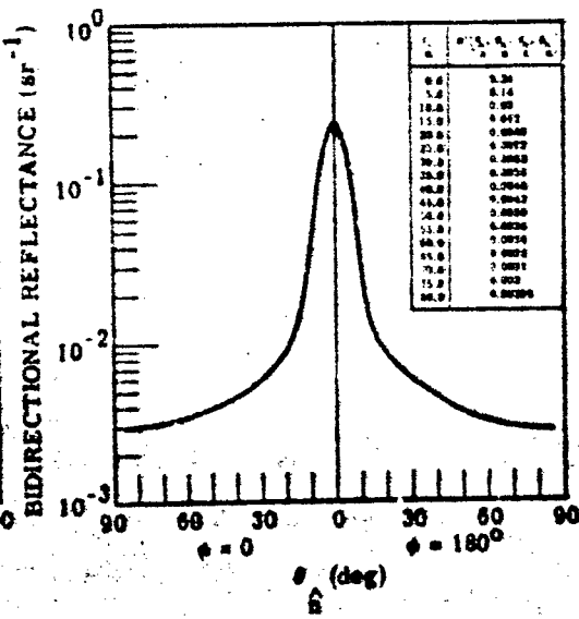
FIGURE 56. FIXED BISTATIC \rho' FOR A01608; \lambda = 0.63 \mu\text{m} .
