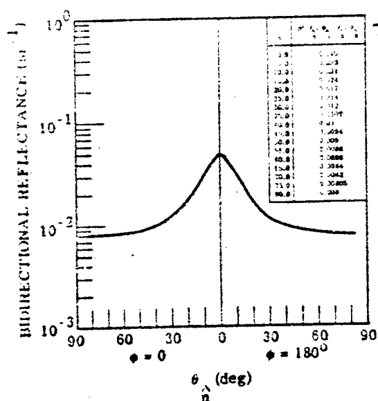
FIGURE 53. FIXED BISTATIC \rho' FOR A01455; \lambda = 0.63 \mu\text{m} .
