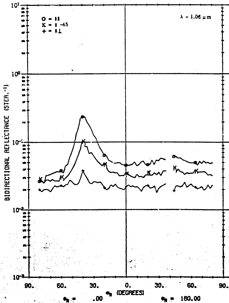
FIGURE 26. MEASURED \rho' FOR A02018-002. \theta_1 = 40^\circ , \phi_1 = 180^\circ , \phi_r = 0^\circ, 180^\circ .
