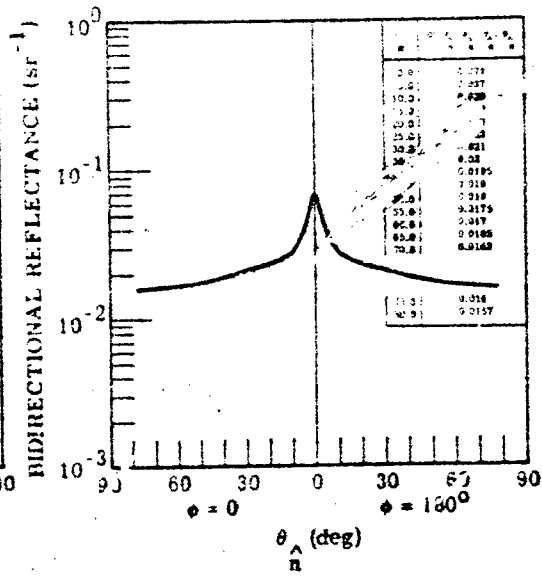
FIGURE 53. FIXED BISTATIC \rho' FOR A01455; \lambda = 0.63 \mu\text{m} .
