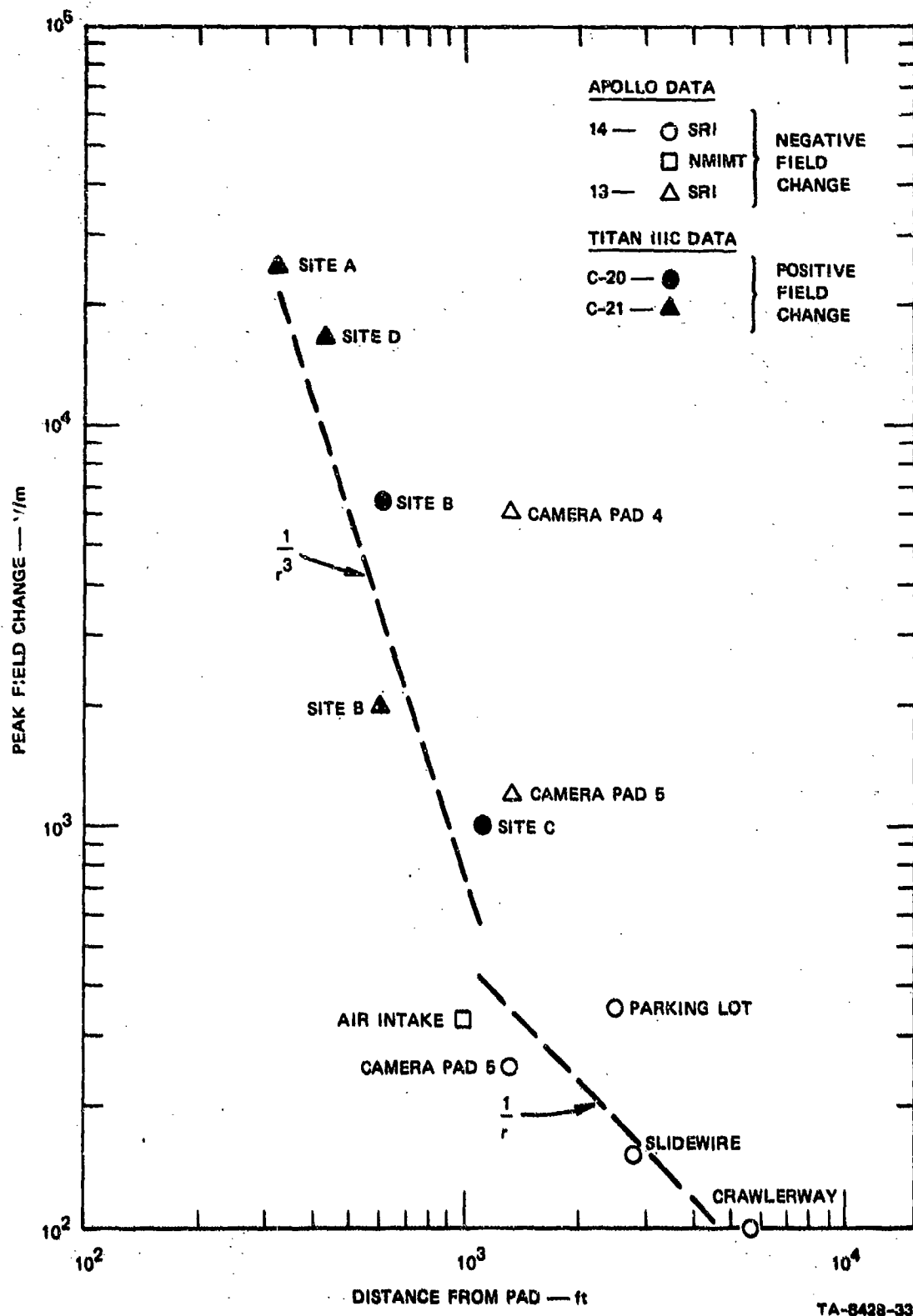
FIGURE B-11 COMPARISON OF MAXIMUM FIELD CHANGES FOR APOLLO AND TITAN LAUNCHES
