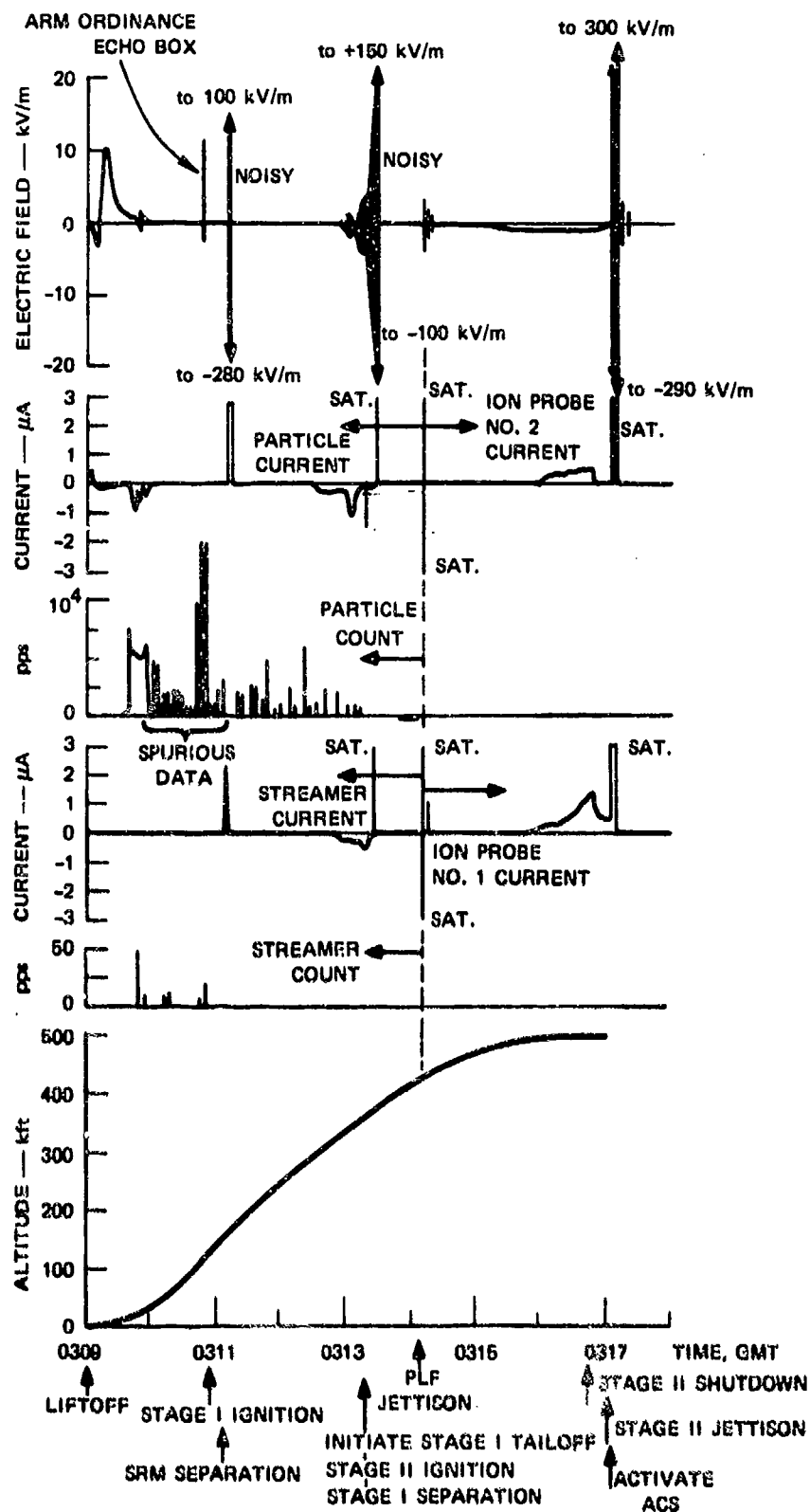
FIGURE 18 TITAN IIC-21 FLIGHT TO 600,000 FT
