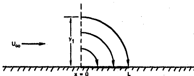
FIGURE C-1 ION-PROBE GEOMETRY
