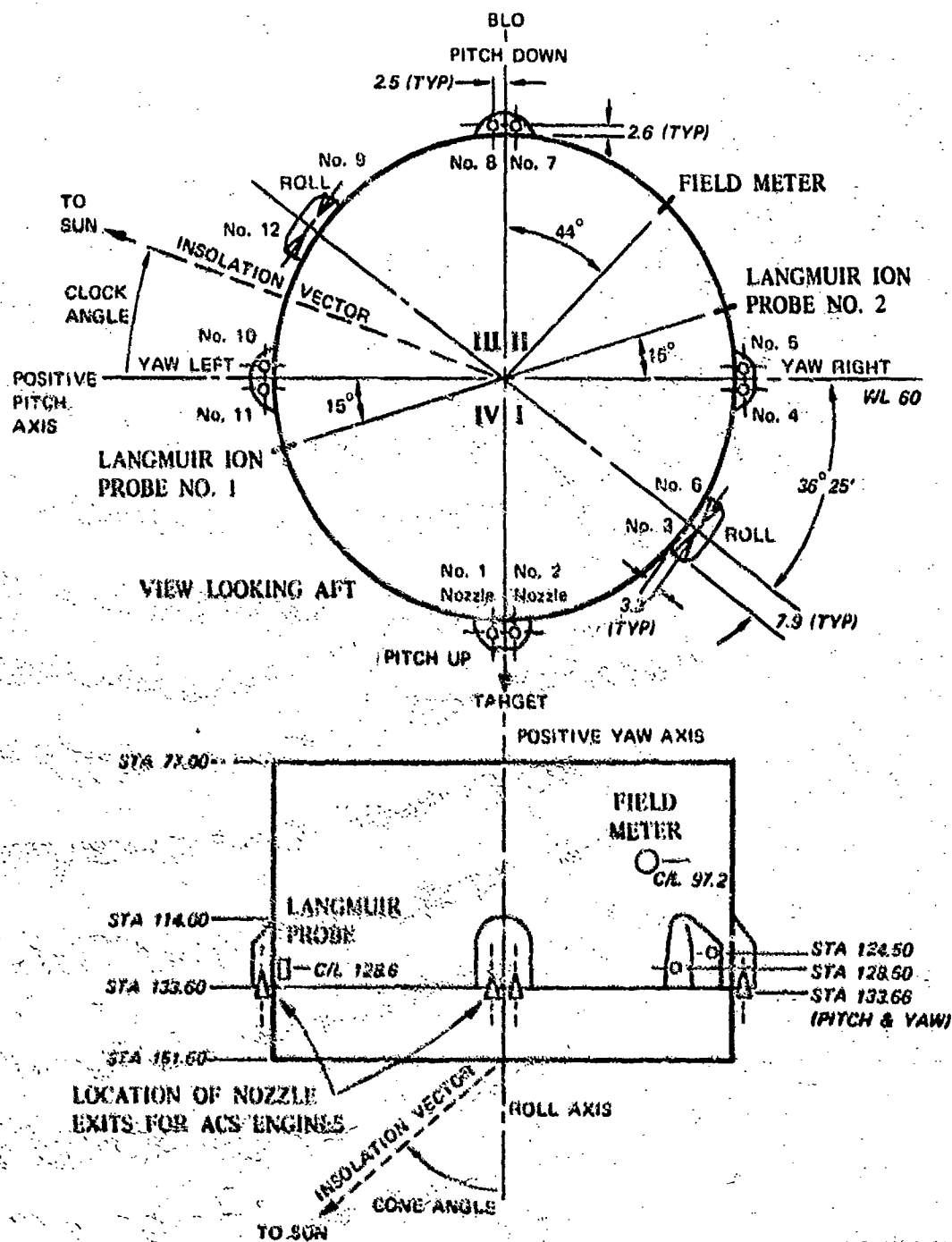
FIGURE D-1 PLACEMENT OF SENSORS AND ALTITUDE-CONTROL ROCKETS ON TITAN III C TRANSTAGE
