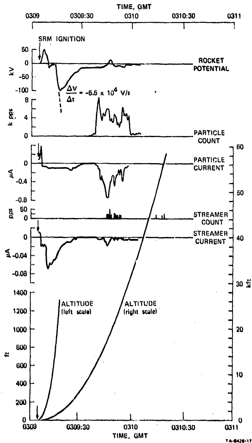
FIGURE 11 LAUNCH DATA FROM TITAN IIIC-21
