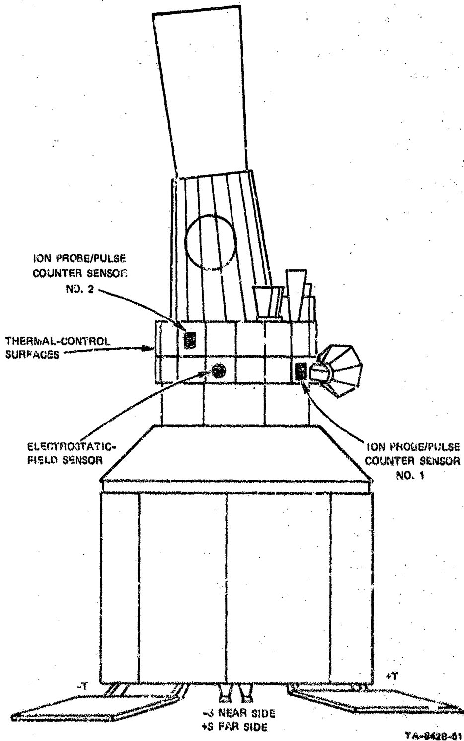
FIGURE 3-2 STANFORD RESEARCH INSTITUTE SENSOR LOCATIONS
