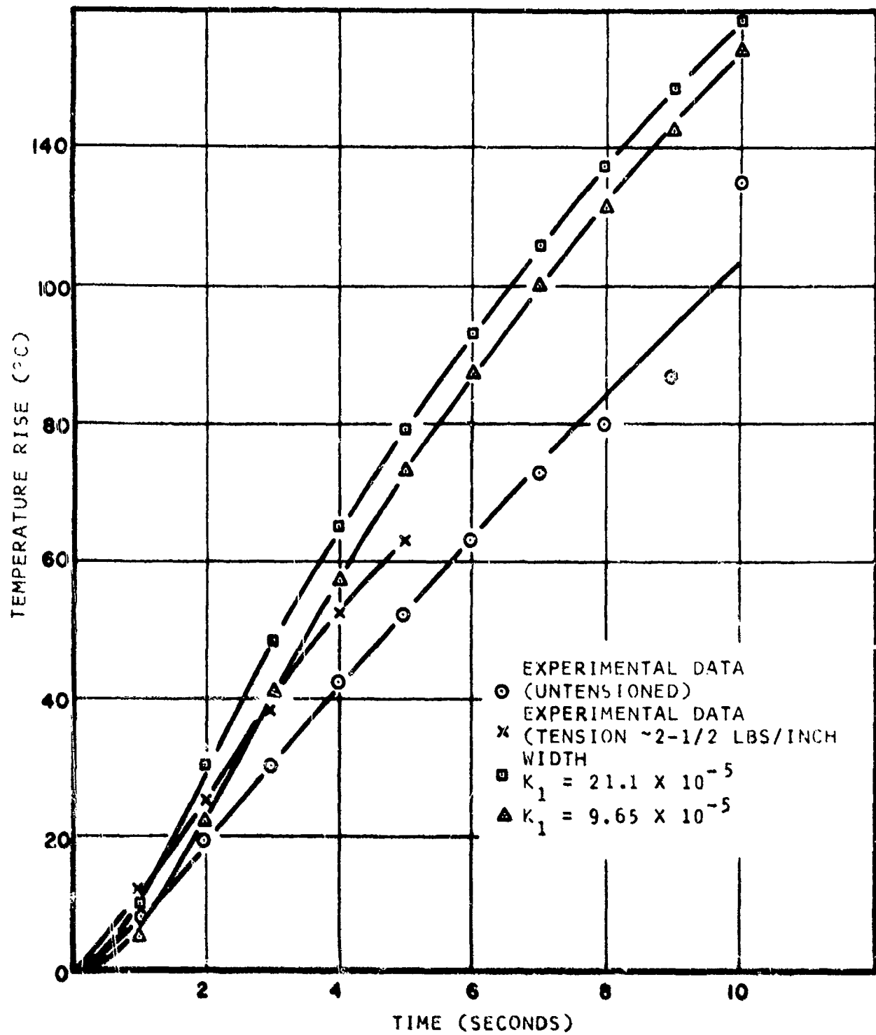
Figure 9. Temperature Rise in Skin Simulant Through Spun Nomex Fabric (AFML#1)
