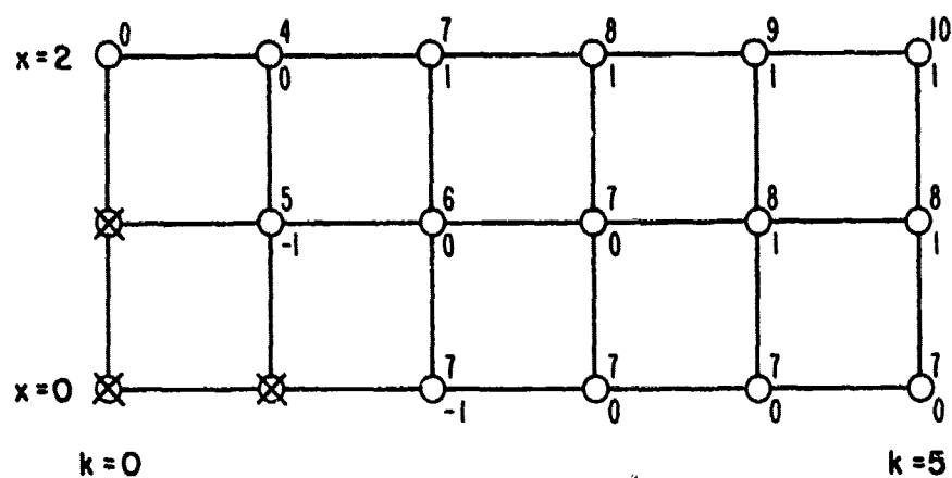
FIG. 4 COMPLETE RESULTS FOR FORWARD DYNAMIC PROGRAMMING EXAMPLE
