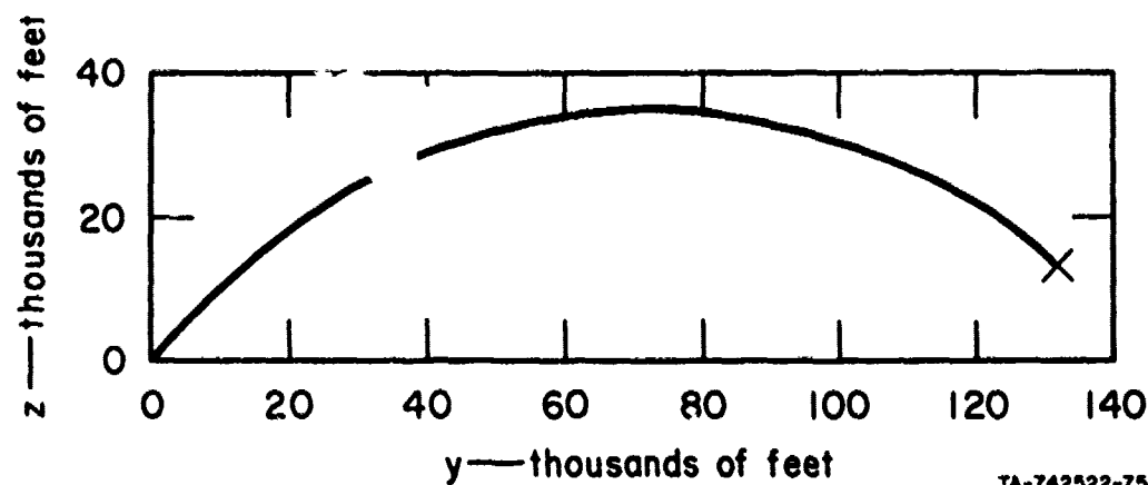
FIG. 8 REPRESENTATIVE MINIMUM-TIME TRAJECTORY TO (y,z) = (131000, 12900)
