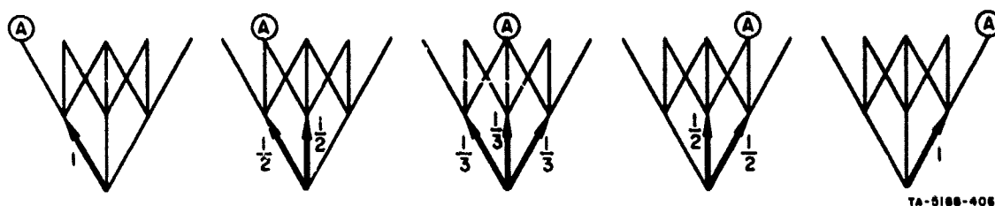
FIG. 6 INTERCEPTOR OPTIMAL CONTROL LAW WHEN INTERCEPTOR REMAINS ON GROUND FOR TWO UNITS OF TIME
