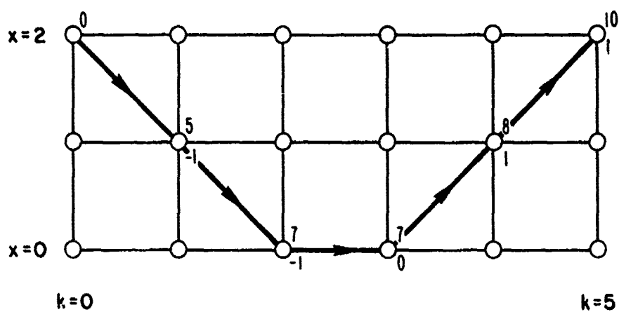
FIG. 5 OPTIMAL TRAJECTORY IF FINAL STATE MUST BE x = 2
