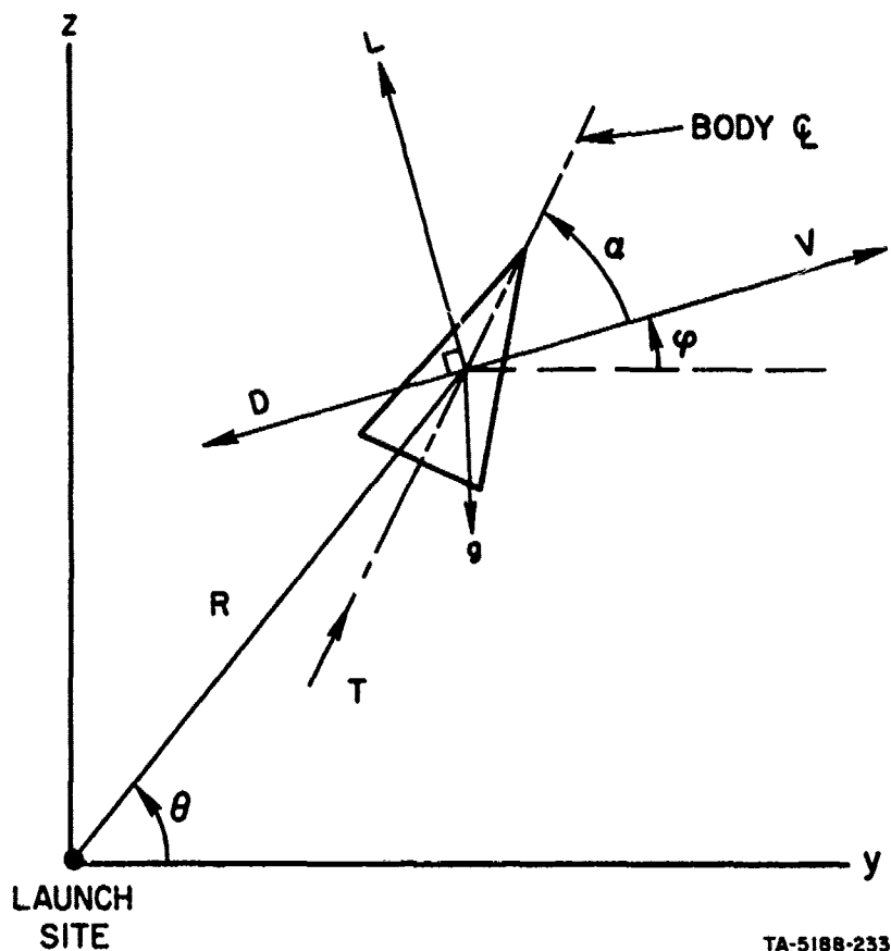
FIG. 7 MISSILE GEOMETRY
