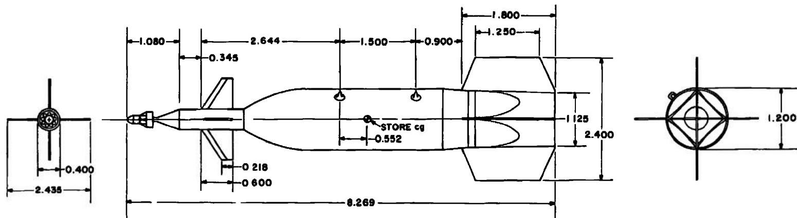
Fig. 10 M-118 Laser Guided Bomb Store
