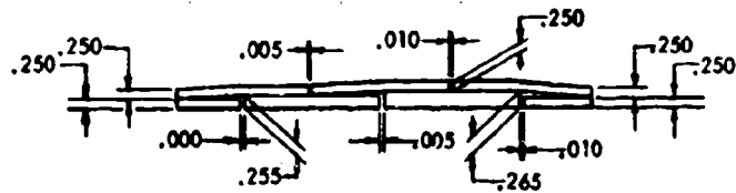
Figure 118 BRAZING TEST PANEL WITH BUILT-IN VOIDS
