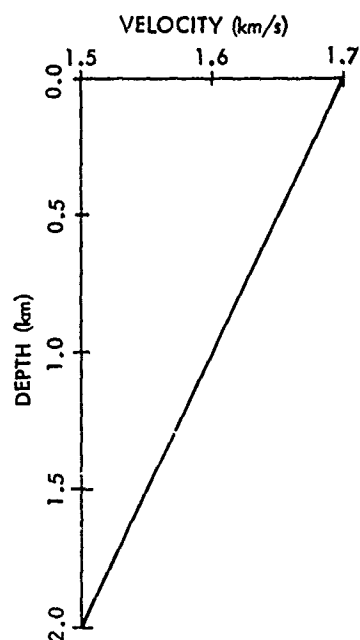
Figure 15. Half-Space in Which the Velocity Decreases with Depth
