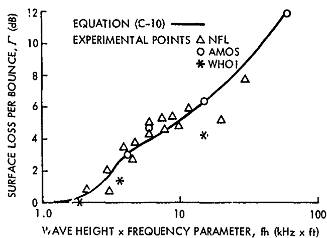
Figure C-1. Surface-Reflection-Loss Curve
