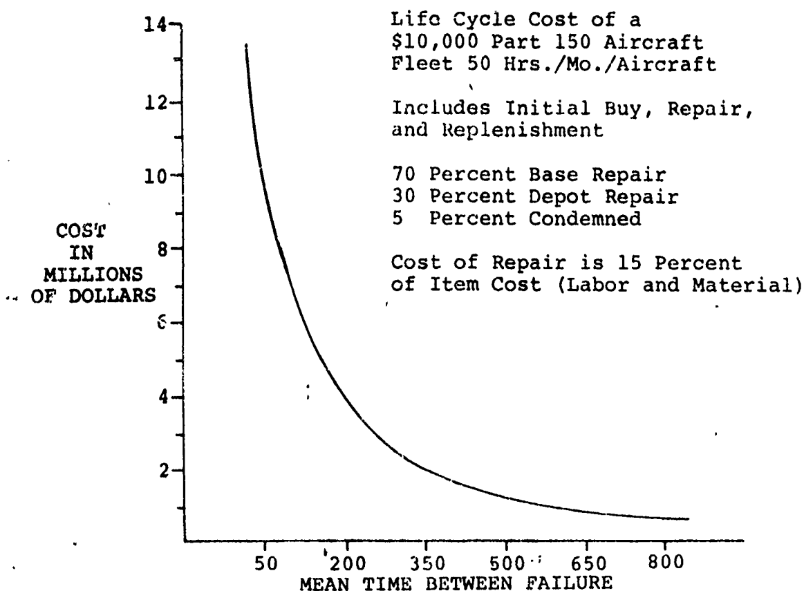
Figure 17: RELIABILITY VERSUS SPARES COST
