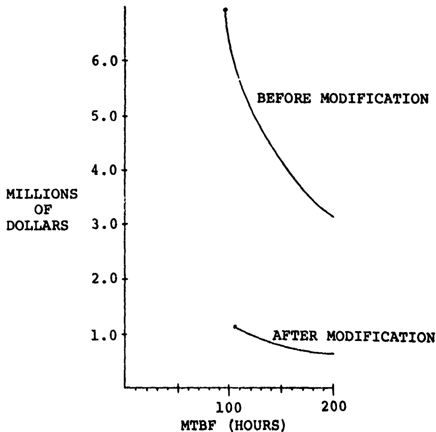
Figure 29: A-7D AIR DATA COMPUTER TEN-YEAR LOGISTIC SUPPORT COSTS VERSUS MTBF
