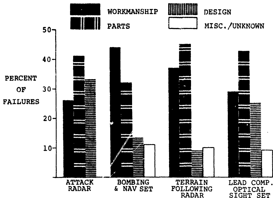
Figure 15: F-111-4 EARLY AGREE TEST PART FAILURE DISTRIBUTION
