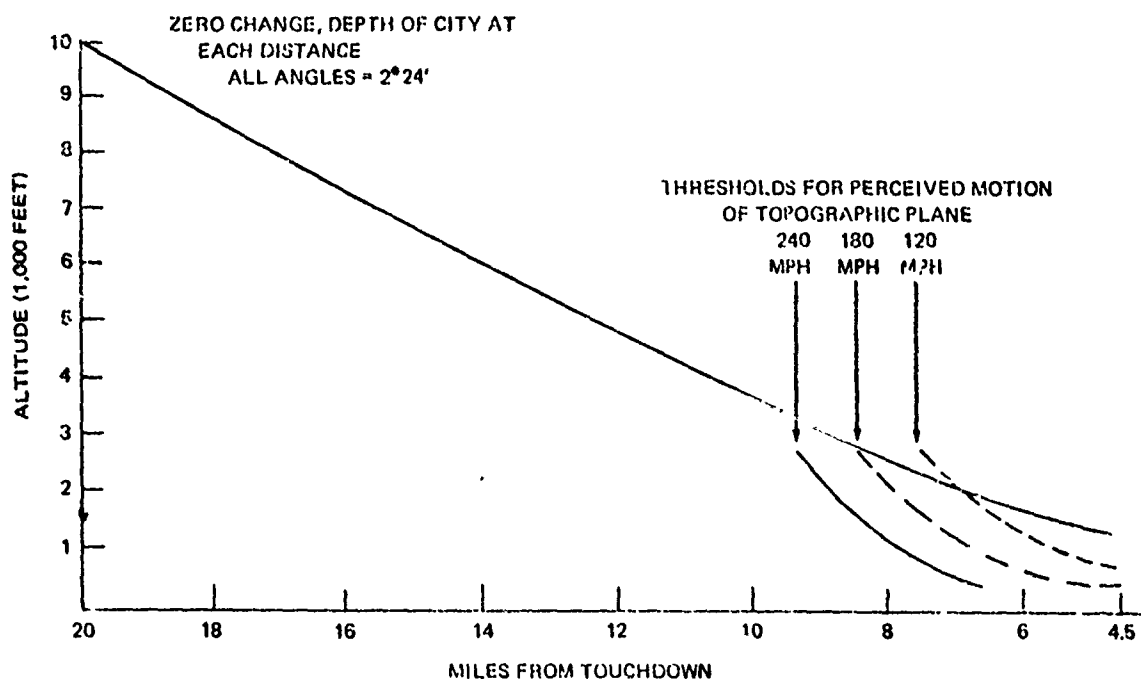
Figure 22: ZERO CHANGE APPROACH PATH AND THRESHOLDS PERCEIVED MOTION
