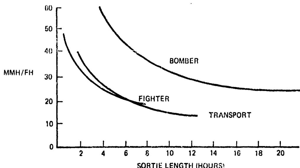
Figure 7: MAINTENANCE MANHOUR - SORTIE LENGTH TREND
