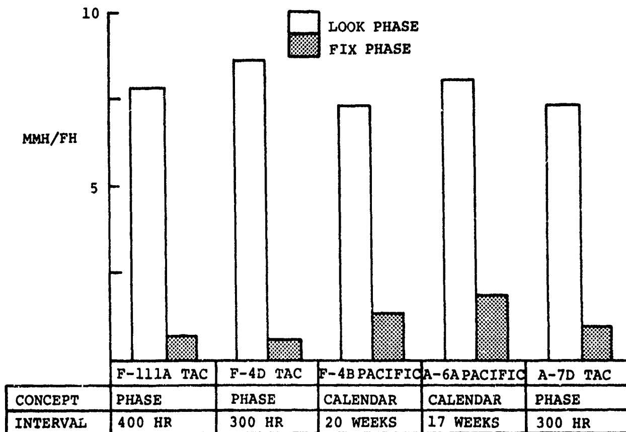
Figure 9: LOOK AND FIX MAINTENANCE COMPARISON
