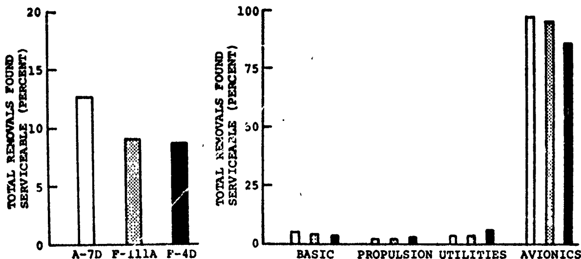
Figure 11: SERVICEABLE REMOVALS
