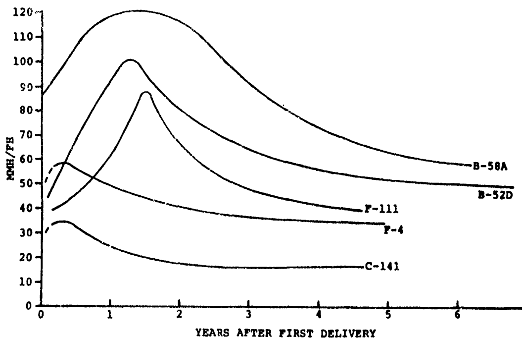
Figure 6: MAINTENANCE GROWTH
