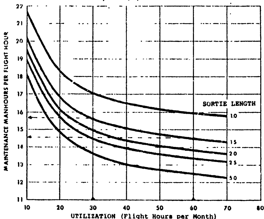
Figure 8: F-4 MMH/FH VERSUS SORTIE LENGTH AND UTILIZATION
