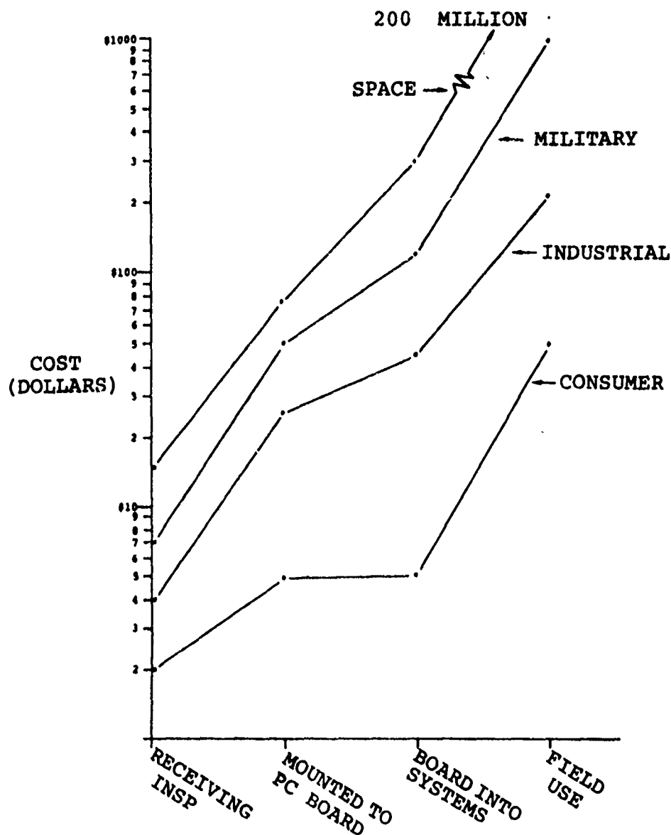
Figure 14: INTEGRATED CIRCUIT REPLACEMENT COST
