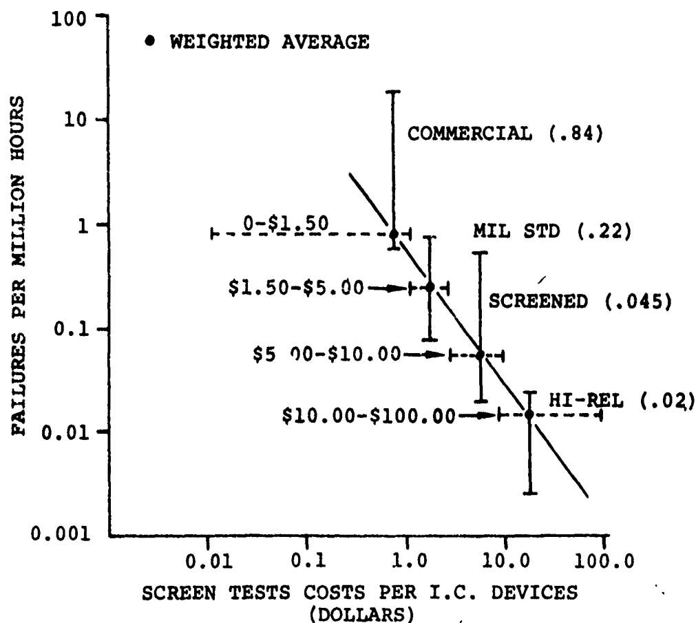
Figure 13: INTEGRATED CIRCUIT QUALITY LEVELS VERSUS COST TO ACHIEVE
