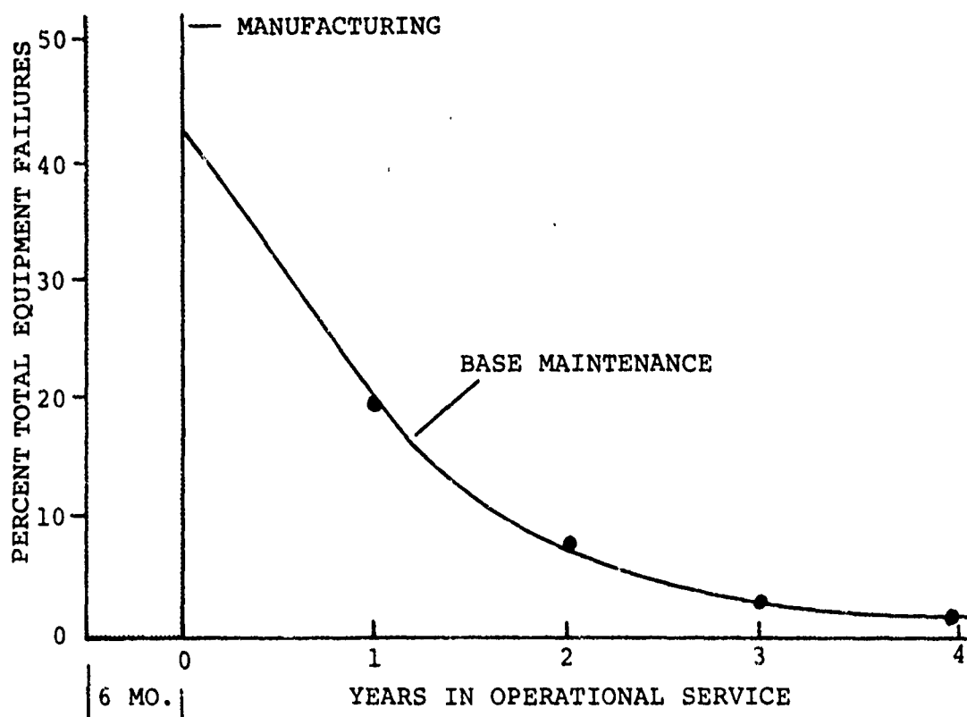
Figure 21: WORKMANSHIP IMPACT ON EQUIPMENT FAILURE
