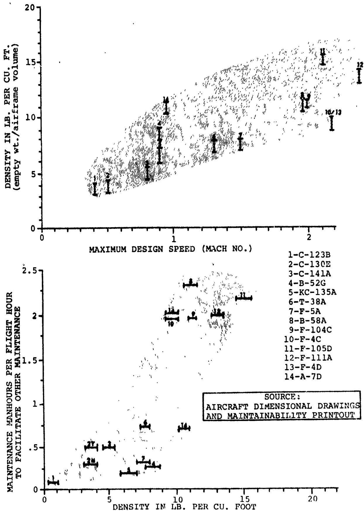
Figure 10: EFFECTS OF EQUIPMENT DENSITY
