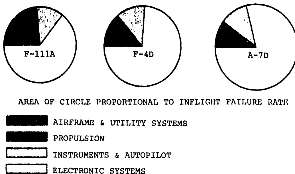
Figure 12: SYSTEM DISTRIBUTION OF INFLIGHT FAILURES
