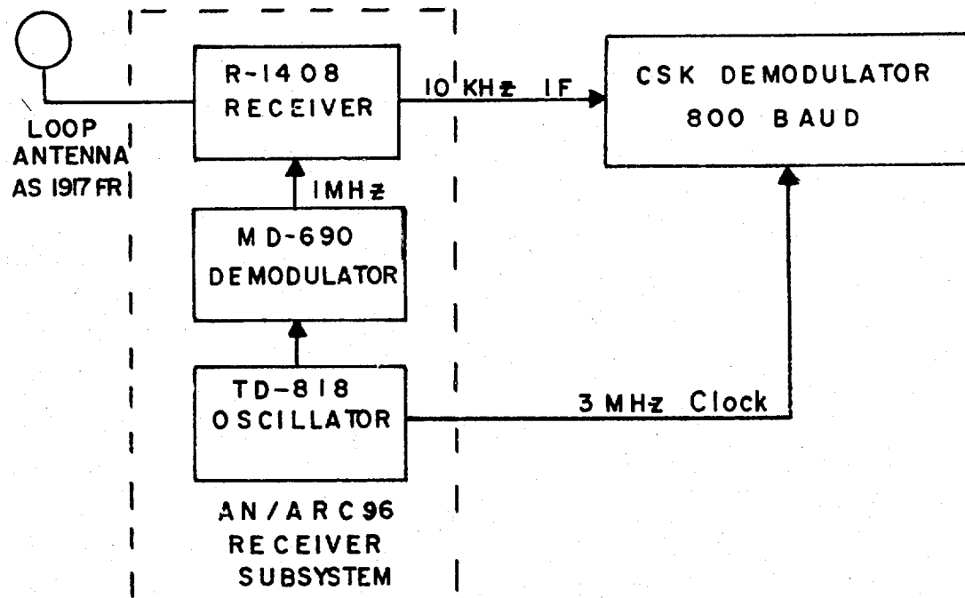
Figure 8. Receiving System
