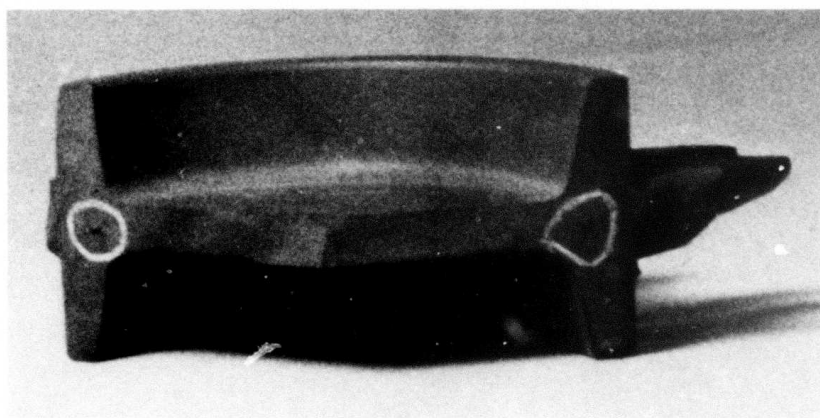
Figure 5.63 Typical Shrink Type Flaws Associated with Injection Molding a Blade Ring and Platform
