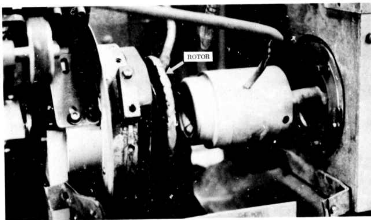
Figure 3.19 Silicon Nitride Rotor Mounted in Ultrasonic Grinding Machine
