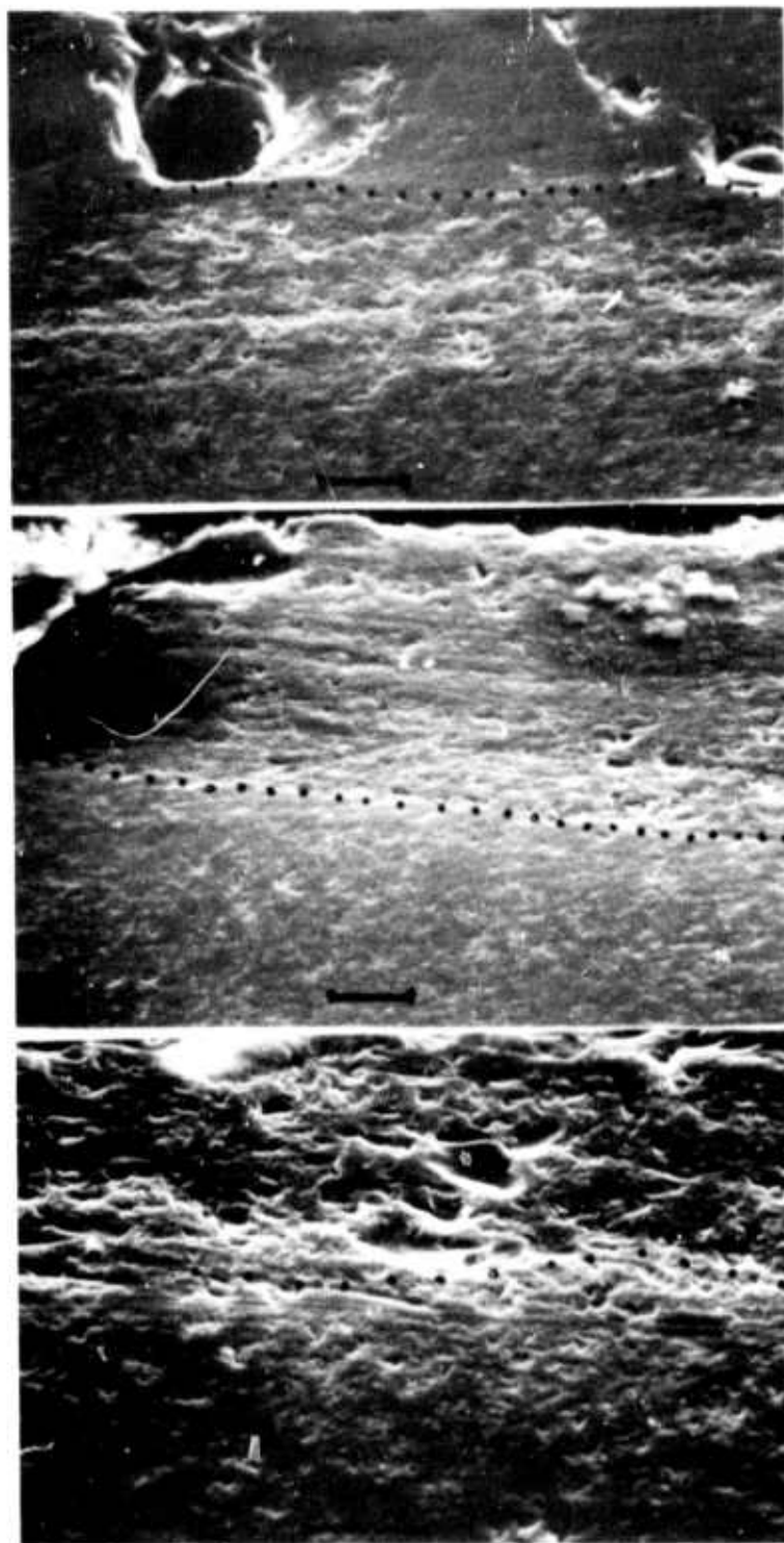
Figure 5.30 SEM Micrographs of Transverse Sections Through the Glass- \text{Si}_3\text{N}_4 Interface for: (a) 80 \text{SiO}_2 ·20 \text{MgO} (b) 95 \text{SiO}_2 ·5 \text{MgO} (c) 95 \text{SiO}_2 ·5 \text{CaO} (Dotted Lines Mark Original \text{Si}_3\text{N}_4 Surface, 20 \mu\text{m} Scale)
