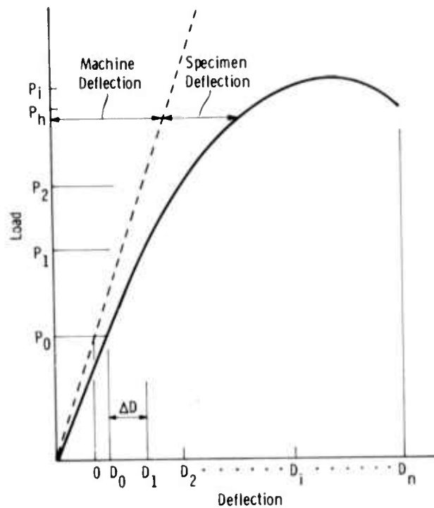
Figure 5.11 Treatment of a Measured Load-Deflection Curve
