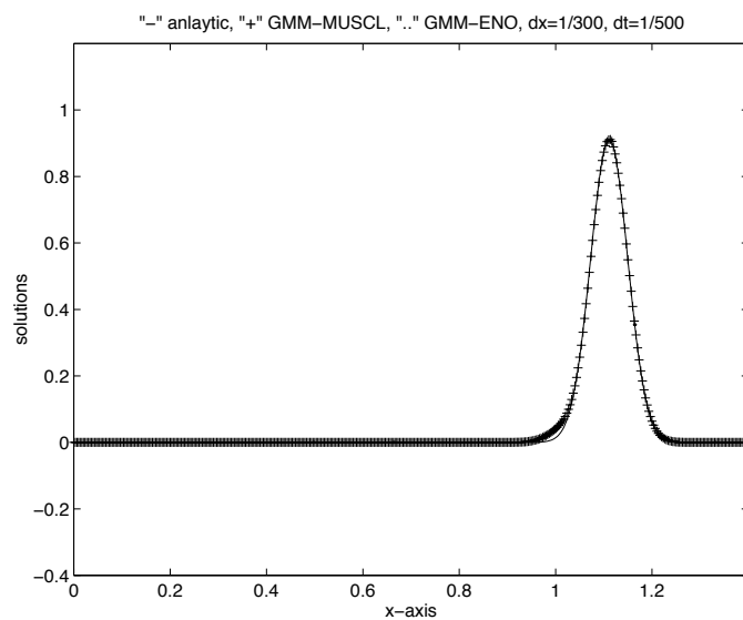
Fig I.5 High resolution methods MUSCL and ENO
