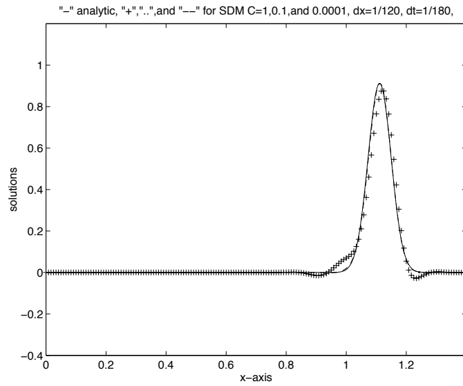
Fig I.3 Streamline Diffusion Method, C = 1, 0.1, \& 0.0001
