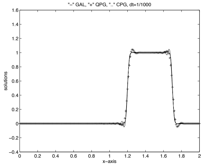
Fig II.2 Galerkin, quadratic and cubic Petrov-Galerkin
