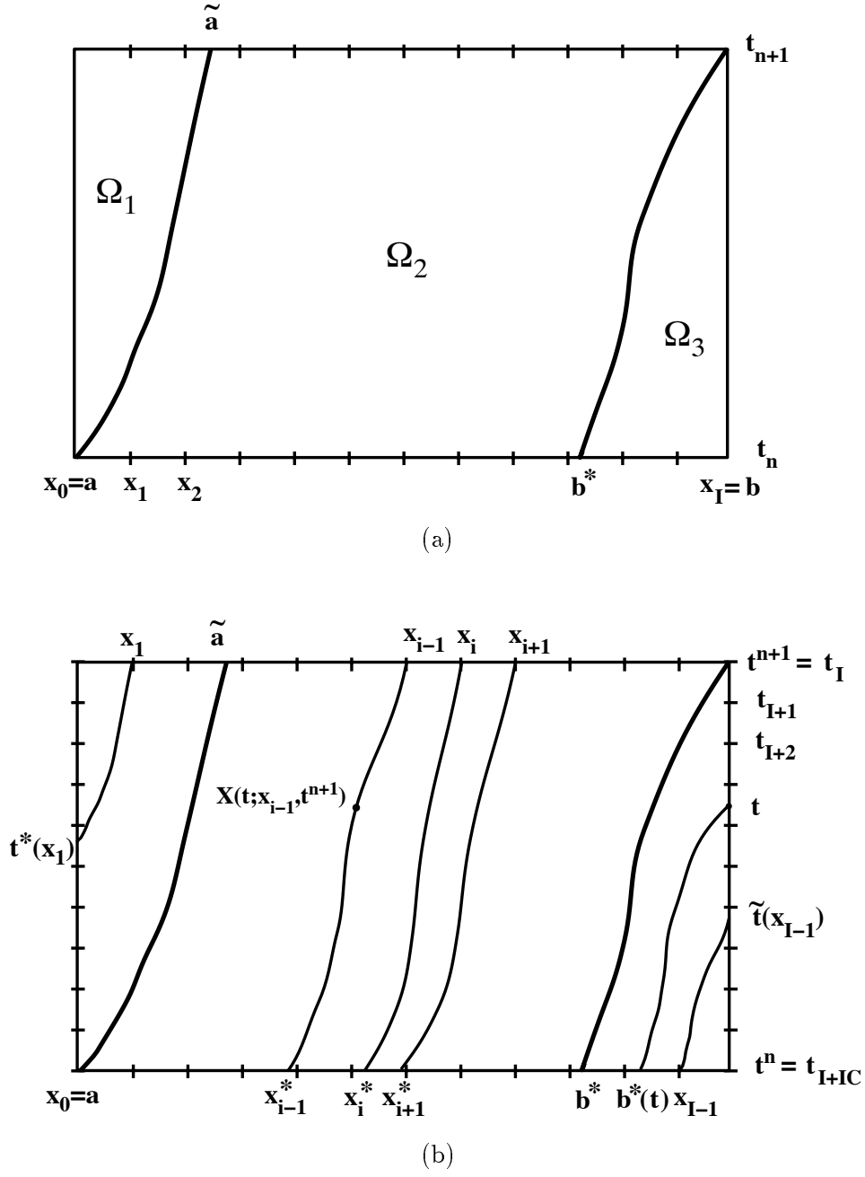
Fig 1. Partition of \Omega (a) The three subdomains \Omega_i ( i = 1, 2, 3 ), (b) Heads and feet of characteristics.
