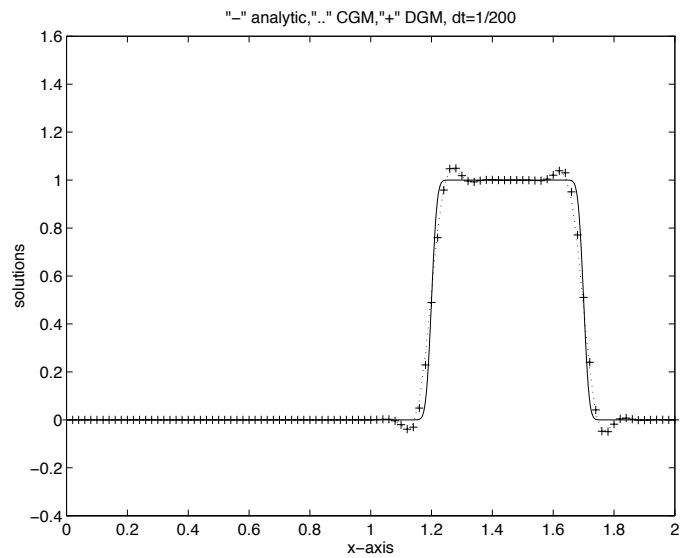
Fig II.4 Continuous and discontinuous Galerkin methods
