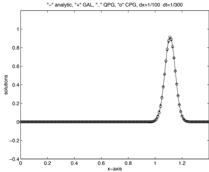
Fig I.2 Galerkin, quadratic and cubic Petrov-Galerkin
