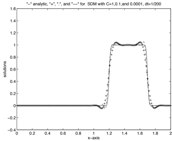
Fig II.3 Streamline Diffusion Method, C = 1, 0.1, \& 0.0001
