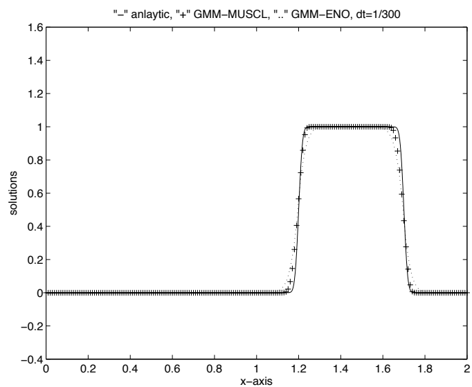
Fig II.5 High resolution methods MUSCL and ENO
