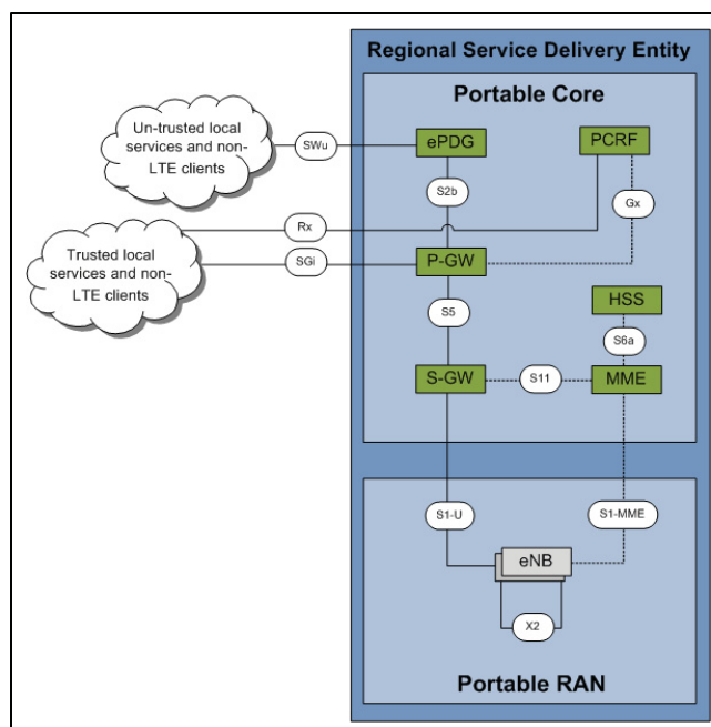
Figure 4-9: Rapidly Deployable Network without Backhaul Link
