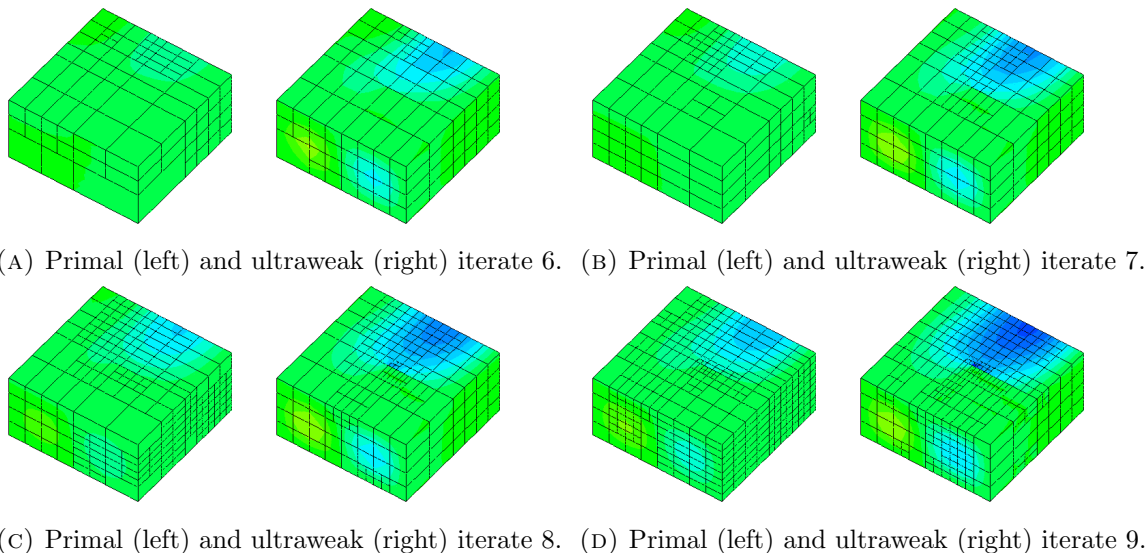
FIGURE 8. Same scale comparison of real part of E_1 computed by the primal and the ultraweak formulations. A middle slice (through singular vertex) of adaptive iterates 6,7,8 and 9 are shown.
