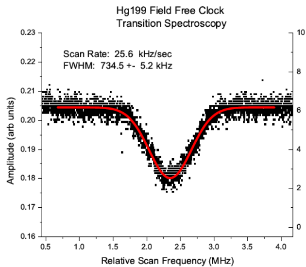
Figure 3. Spectroscopy of the \text{Hg}^{199} clock transition in the absence of the MOT beams.
