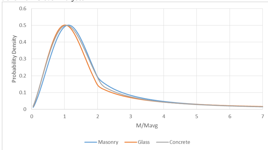
Figure 41 Overlay of average modified Weibull distribution fits
