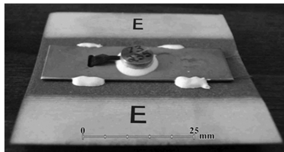
Figure 3 A wireless stress and temperature sensor showing the diaphragm and the mounting shim.
