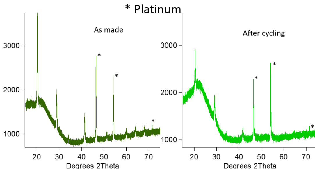
Figure 4.11. X-ray diffraction patterns of a CuHCF electrode after being cycled \sim 20 times in 1M aluminum/diglyme electrolyte. There is clear loss of peak intensity as well as an amorphous bump at low 2Theta. The data indicate dramatic loss of crystallinity of the CuHCF crystal structure after repeated electrochemical cycling.
