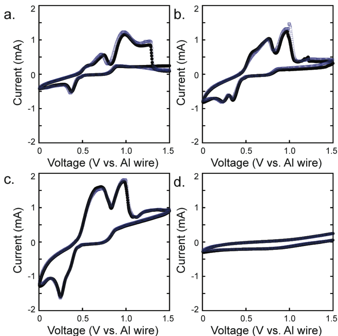
Figure 2.1. Typical jar cell cyclic voltammograms in a 1.2:1 mol/mol AlCl_3 :EMIC electrolyte showing the second (solid black) and fifth (hollow blue) scans on a) a 90:5:5 by weight V_2O_5 :carbon black:pVDF on stainless steel cathode; b) a 50:25:25 by weight V_2O_5 :carbon black:pVDF on stainless steel cathode; c) a 25:37.5:37.5 by weight V_2O_5 :carbon black:pVDF on stainless steel cathode; and d) a 90:5:5 by weight V_2O_5 :carbon black:pVDF on platinum cathode, all at 1mV/s scan rate.
