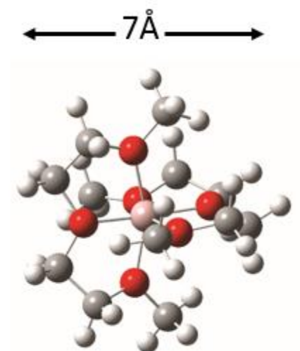
Figure 4.6. The Guassian predicted size of the aluminum/diglyme complex is approximately 7Å. Because of the high stability of the complex it is unlikely that any significant desolvation of the \text{Al}^{3+} occurs during intercalation. Thus, it is likely that the entire complex intercalates/de-intercalates during cycling.
