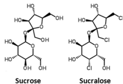
Figure 3. Sucralose and sucrose have similar chemical structures. Sucralose contains chlorine atoms at three positions, in place of the oxygen atoms found in sucrose. (Chemspider 2013)
