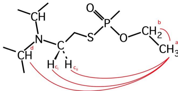
Figure 9. Dipolar-coupled proton pairs in VX. The four dipolar-coupled proton pairs (red lines) identified in this effort for aqueous VX were (1) the H_a – H_b pair, (2) the H_a – H_{ci} pair, (3) the H_a – H_{cii} pair, and (4) the H_a – H_d pair.
