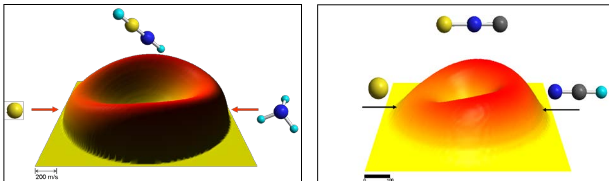
Figure 1. Flux contour map of the imidoborane molecule ( \text{HNBH} ) (left) and boronisocyanide ( \text{BNC} ) (right) formed in the reaction of atomic boron, ^{11}\text{B}(^2P_1) , with ammonia, \text{NH}_3(X^1A_1) , and hydrogen cyanide ( \text{HCN}(X^1\Sigma^+) ) at collision energies of 20.5 \text{ kJmol}^{-1} and 29.2 \text{ kJmol}^{-1} , respectively.
