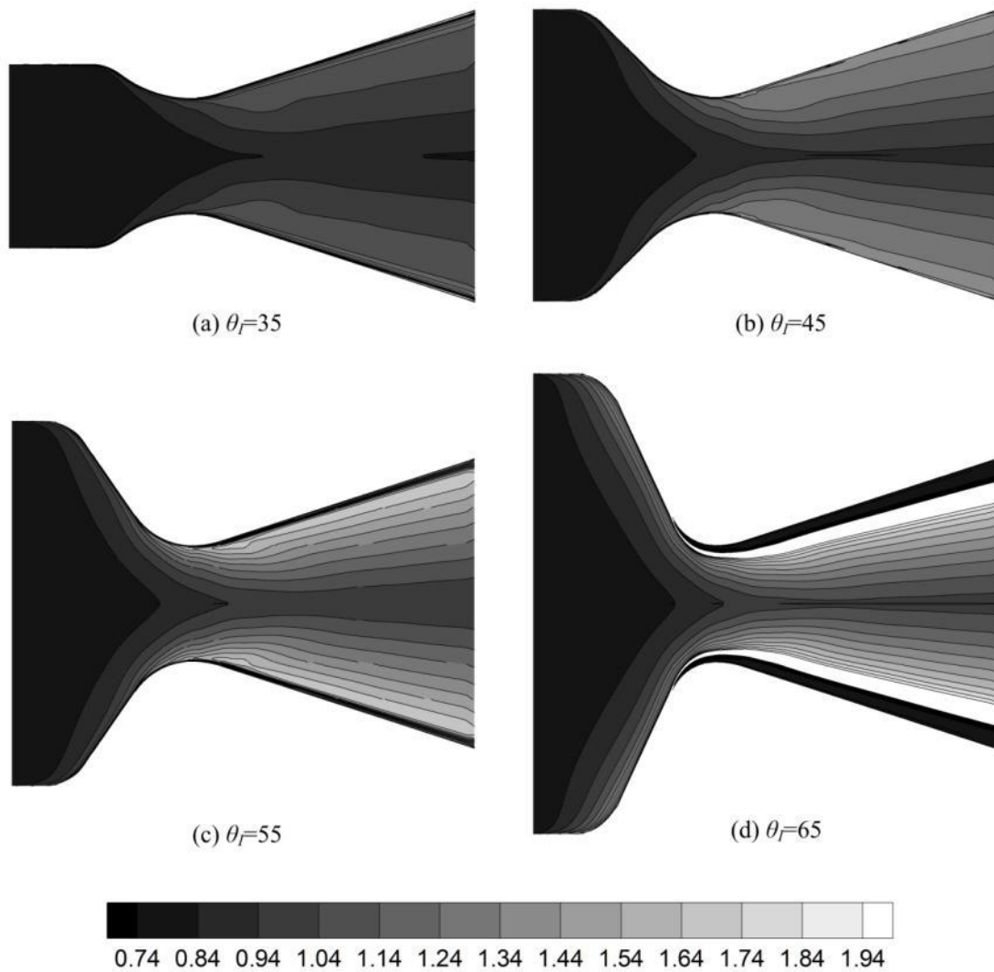
Figure 3.33 Predicted D_{43} contours of the contraction angles from 35 to 65 deg. for I-1 to 4
