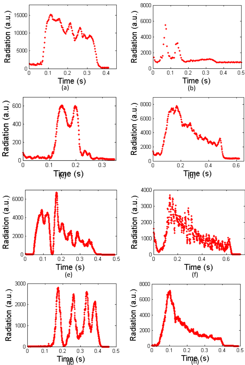
Fig. 10 AIO emission (radiation) plots over time for droplets burning in compressed air at 1000 psi for all fuel mixture variations used in systematic study. All mixtures are nitromethane with the following loadings: (a) baseline mixture (4 wt.% 80 nm Al 1 wt.% Aerosil 380) (b) 4 wt.% 30 \mu m Al 1 wt.% Aerosil 380 (c) 4 wt.% 100 nm Al 1 Wt.% Aerosil 380 (d) 4 wt.% 38 nm Al 1 wt.% Aerosil 380 (e) 6 wt.% 80 nm Al 1 wt.% Aerosil 380 (f) 2 wt.% 80 nm Al 1 wt.% Aerosil 380 (g) 4 wt.% 80 nm Al and no Aerosil 380 (h) 4 wt.% 80 nm Al 2 wt.% Aerosil 380.
