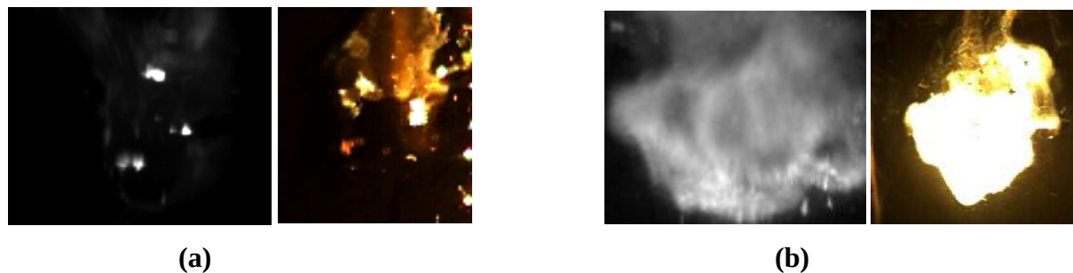
Fig. 8 Phases of combustion of the 4 wt.% 80 nm Al 1 wt.% Aerosil 380 Nitromethane through the 486 nm notch filter (left) and the full color spectrum (right). Part (a) shows the first stage of the burn, with light aluminum participation, while part (b) shows the typical second stage of the burn, which had a much more extensive aluminum participation in the burn.
