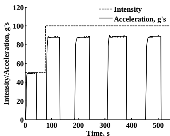
Fig. 4 Sample mixing Resodyn LabRam data for ethanol with 1 wt.% nAl.
