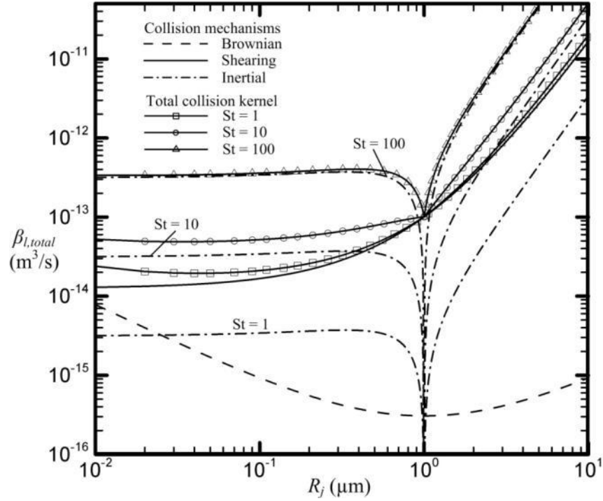
Fig. 9 Comparisons of total collision frequency functions for various Stokes numbers (R_i = 1 \mu\text{m}, T = 3000 \text{ K}, \mu = 36\text{e-}5 \text{ kg/m-s}, \rho_p = 1000 \text{ kg/m}^3, s'_{xx} = s'_{yy} = s'_{zz} = -1000 \text{ 1/s})
