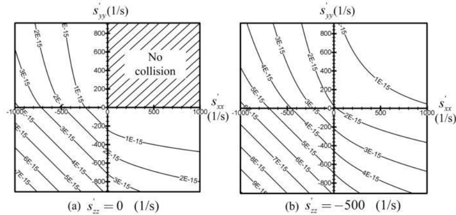
Fig. 4 The shearing collision frequency function contours for R_c = 1 \mu\text{m} (units: \text{m}^3/\text{s} ); (a) s'_{zz} = 0 and (b) s'_{zz} = -500 \text{ 1/s}
