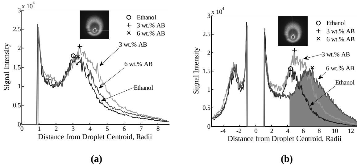
Figure 21 Horizontal, (a), and vertical, (b), slices taken from images in Figure 20 showing the OH PLIF signal as a function of droplet radius. The signal from the droplet itself is removed from the figures by giving it a value of zero. The o, +, and x markers correspond to the peaks in the OH reaction zone.
