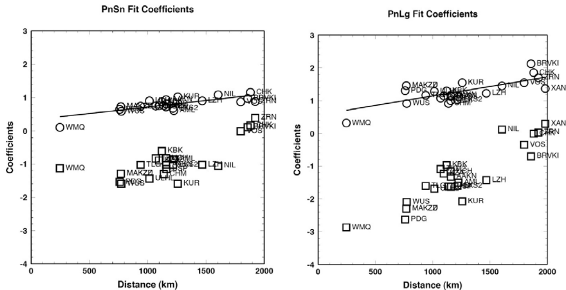
Figure 14. Slopes (circles) and intercepts (squares) of Pn/Sn (left) and Pn/Lg (right) spectral ratios for regional paths from LNTS.
