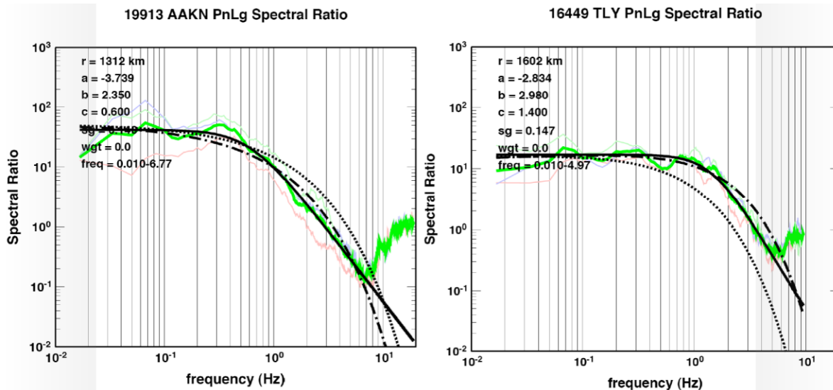
Figure 13. Lg/Pn spectral ratios and comparisons to Q predictions for two paths, (left) from southwestern Siberia to KNET station AAK and (right) from LNTS to station TLY.
