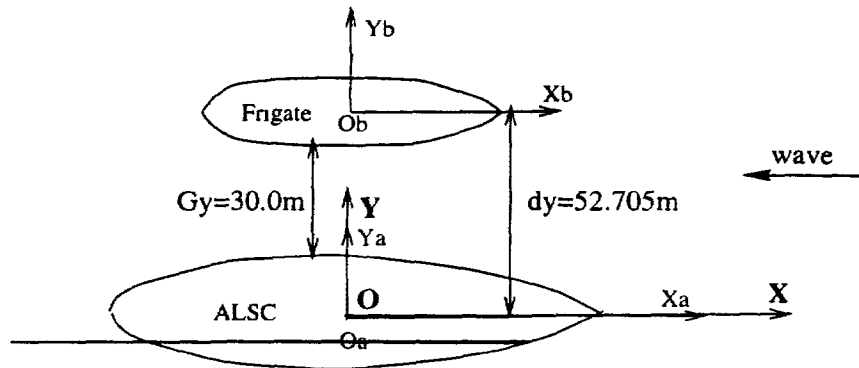
Figure 6: Separation Distance of Two Ships: G_y=30.0 m, dx=0.0 m
