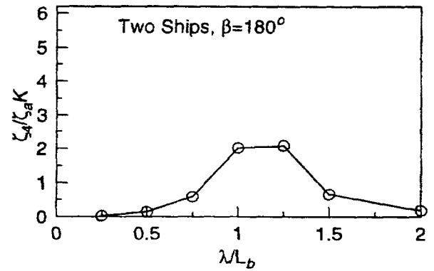
Roll motion of Frigate at a separation Gy=30.0m dx=0.0m U=0.0m/s
