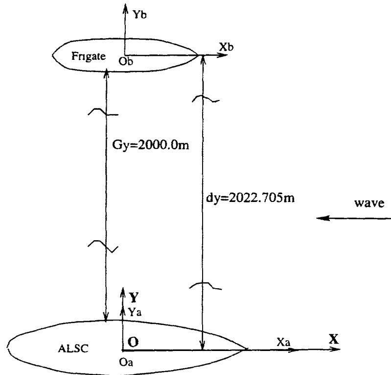
Figure 18: Separation Distance of Two Ships: Gy=2000.0m , dx=0.0m
