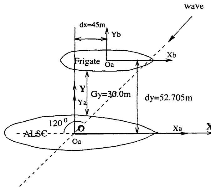
Figure 36: Separation Distance of Two Ships: Gy=30.0\text{m} , dx=45.0\text{m}
