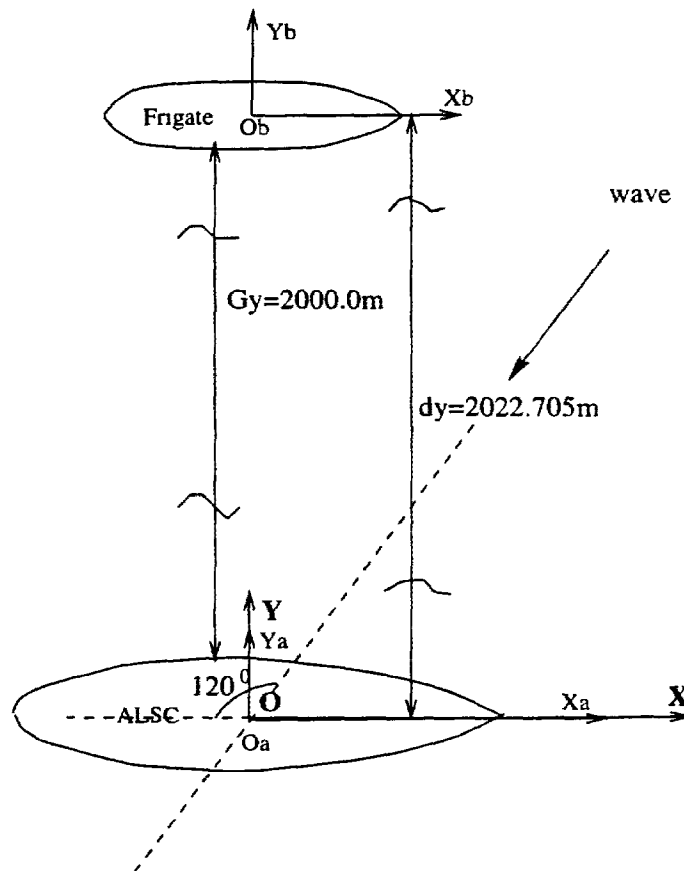
Figure 39: Separation Distance of Two Ships: Gy=2000.0\text{m} , dx=0.0\text{m}
