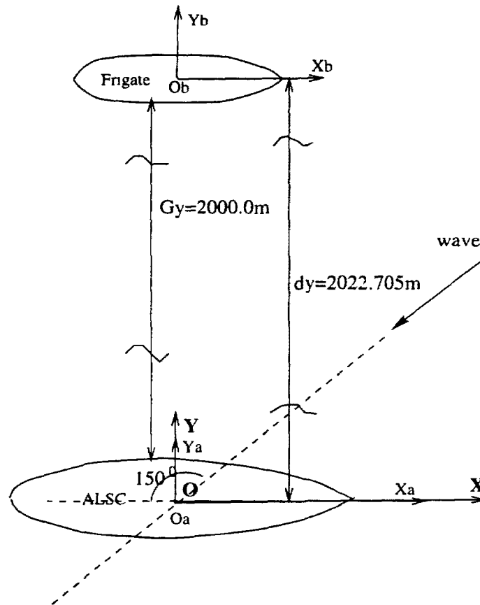
Figure 30: Separation Distance of Two Ships: Gy=2000.0\text{m} , dx=0.0\text{m}
