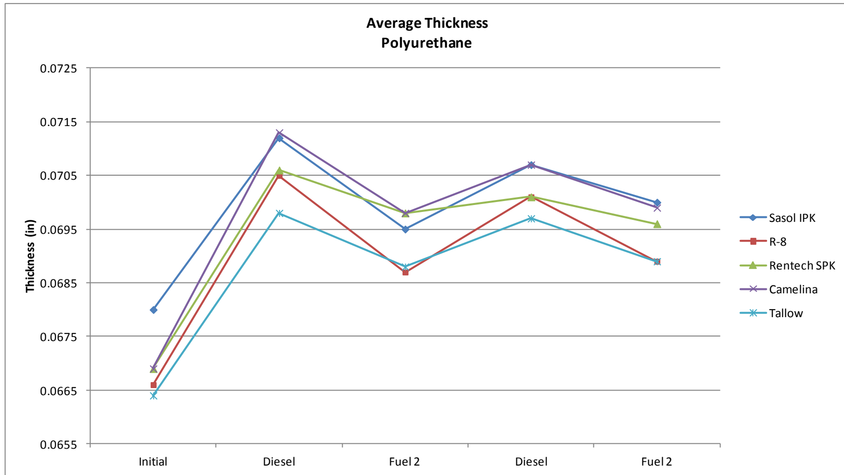
Figure 46. Thickness Data for Polyurethane Switch-Loading Samples after 8 Weeks with Diesel as the Baseline Fuel
