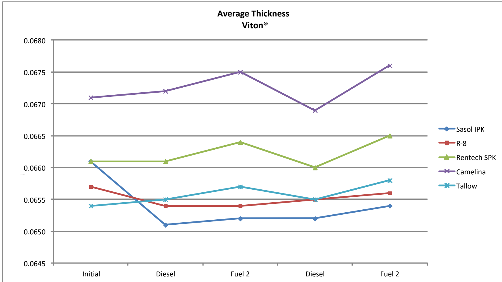
Figure 53. Thickness Data for Viton® Switch-Loading Samples after 8 Weeks with Diesel as the Baseline Fuel
