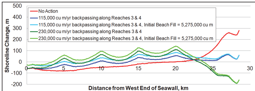
Fig. 14. Total shoreline change after 50 years with 115,000 m 3 and 230,000 m 3 backpassed to Reaches 3 and 4 with and without an initial beach fill.
