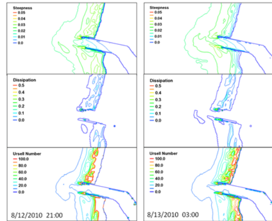
Fig. 18. Calculated wave steepness (top), wave dissipation (middle) and Ursell number (bottom) during a flood current on 12 August 2010 at 21:00 GMT and an ebb current on 13 August 2010 at 03:00 GMT.
