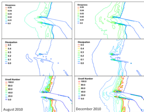
Fig. 16. Calculated monthly mean wave steepness (top), wave
