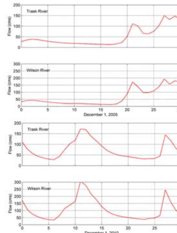
Fig. 10. River flow discharges for December 2005 and 2010 from USGS gages at Trask (#14302480) and Wilson (#14301500) Rivers, Oregon.
