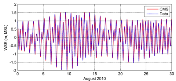
Fig. 11. Calculated water surface elevation at Garibaldi, August 2010.
