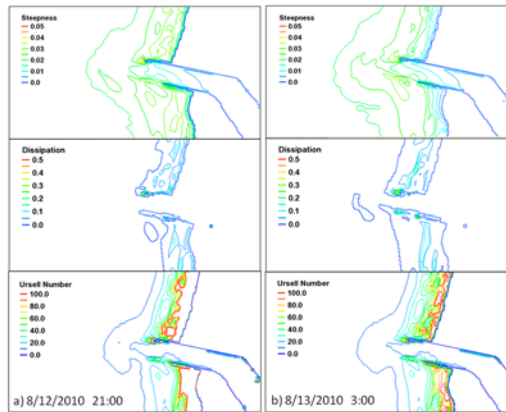
Fig. 25. Wave steepness (top), wave dissipation (middle), and Ursell number (bottom) for the shortened South Jetty: a) flood current in 12 August 2010 at 21:00 GMT and b) ebb current in 13 August 2010 at 03:00 GMT.
