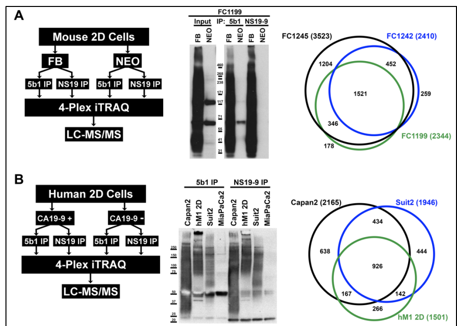
Figure 2. Identification of CA19-9 carriers in monolayer cultures of human and mouse PDAC cells. A. Identification strategy for mouse CA19-9 carriers in cells expressing Fut3 and β3GalT5 (FB). Representative CA19-9 western blot of immunoprecipitation (IP) shown. B. Identification strategy for human CA19-9 carriers and representative IP. Overlap for both mouse and human carriers generated by calling CA19-9 carriers as 1.5-fold up-regulated in CA19-9 positive sample relative to the CA19-9 negative control.
