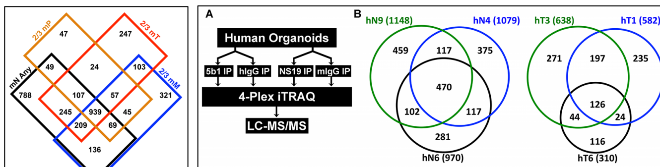
Figure 5. Identification of CA19-9 carriers in human organoids. A. Identification strategy. B. Overlap of CA19-9 carriers identified in hN and hT organoids. CA19-9 carriers are defined as being up-regulated >1.5-fold in the CA19-9 relative to the IgG IP using either CA19-9 antibody.
